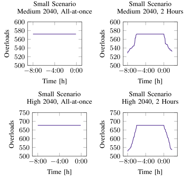
Fig. 12. Overloads per interval for medium and high EV penetration rates in the Small Scenario. In the left column, all the electric vehicles charge simultaneously. In the right column, the vehicle charging start times are randomly assigned over a two-hour window.
