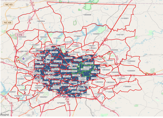
Fig. 5. The TAZs in the area of interest. In total, we have selected 106 TAZs, covering the city center's central area and its surroundings. The colored region contains the buses in the power grid network. The green outlined area denotes the six TAZs we are using in the small evacuation scenario described in Section IV.
