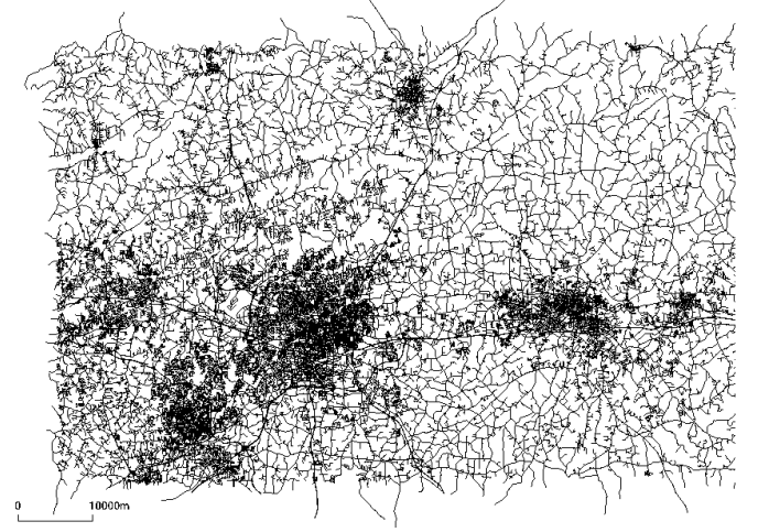
Fig. 4. The road network imported in SUMO.
