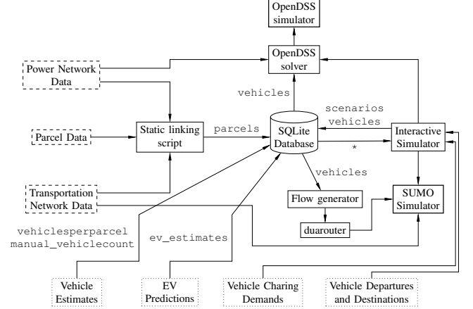
Fig. 9. The detailed architecture of the testbed. The dashed boxes are data obtained from exogenous data sources, while the dotted boxes represent data provided by the user. Next to some of the arrows, the figure indicates which table in the database is used or changed by a script. The simulator utilizes several of the generated tables when creating scenarios with vehicles. These dependencies are denoted an asterisk.
