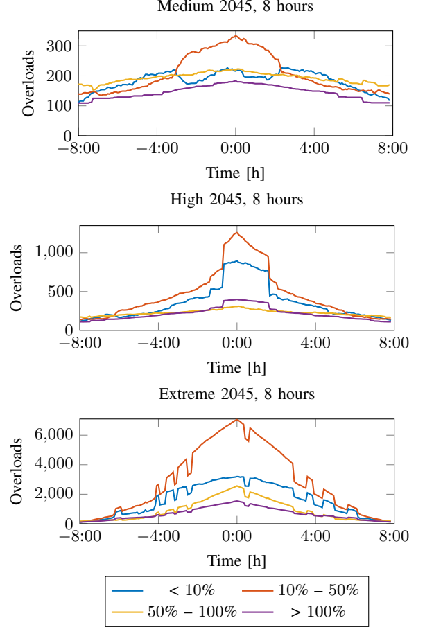
Fig. 17. Overloads under 10% (blue), between 10% and 50% (orange), between 50% and 100% (yellow), and over 100% (purple) for medium, high, and extreme EV penetration rates in the large scenario. Vehicle charging start times are randomly assigned over an eight-hour window.
