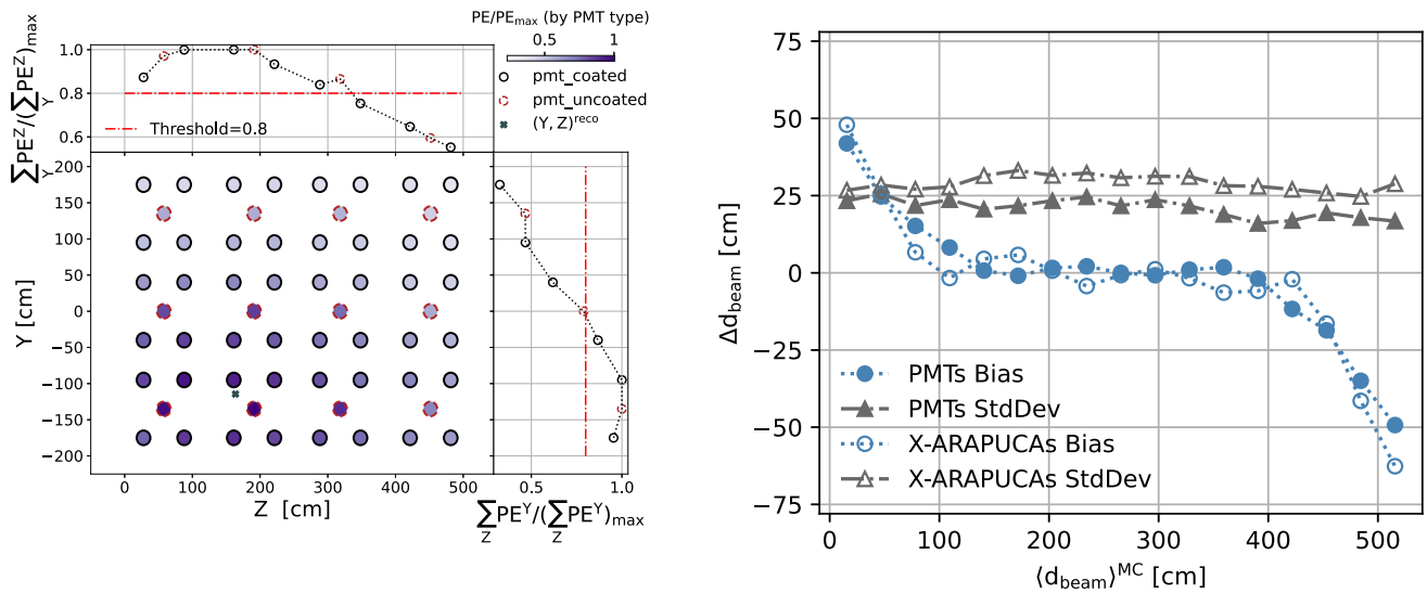
Fig. 11 Left: illustration of the (Y, Z) reconstruction procedure. Right: accuracy and resolution in the estimation of the interaction point in the beam direction ( Z -coordinate) using only scintillation light for PMT
