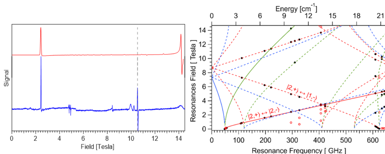
Figure 4. Left: Experimental ( blue ) HFEPR spectrum recorded at 5 K for T using a microwave frequency of 295.2 GHz and theoretical curve ( red ) obtained using the parameters listed in Table 1. The dashed vertical line marks the location of the g = 2.0023 . Right: The black dots present the field vs frequency location of the experimental resonances. The red circles indicate resonances not included in our analysis. The solid curves account for the theoretical dependencies of the ground state resonances and the dashed curves of the excited state resonances. The red, green, and blue colors account for the z , y , and x molecular directions, respectively.
