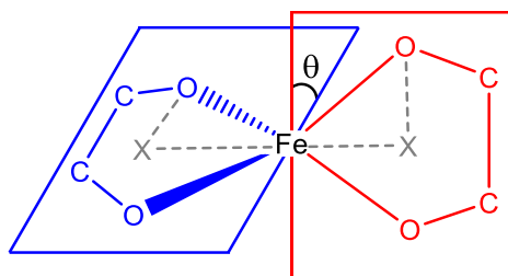
Scheme 3. Definition and measurement of the angle \theta which quantifies the angle formed by the two chelating \text{pin}^{\text{F}} ligands. Thus, \theta is defined with the help of two dummy atoms, labeled X, which are inserted at the midpoint of the O-O distance of each \text{pin}^{\text{F}} ligand such that, numerically, \theta is equal to the resulting OXXO dihedral angle.
