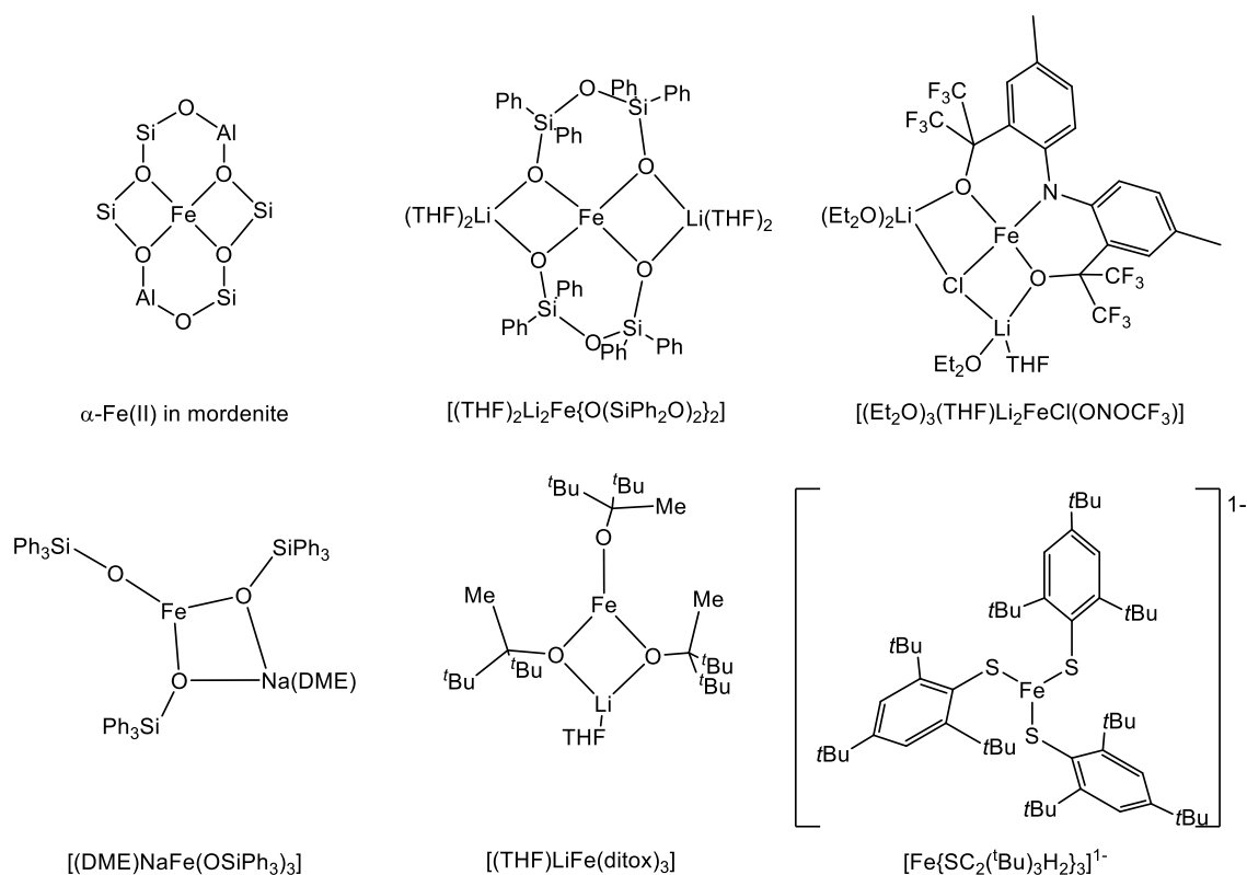
Scheme 1. High-spin Fe(II) complexes which incorporate iron sites with an approximately square planar ( top row ) and trigonal planar ( bottom row ) geometry.
