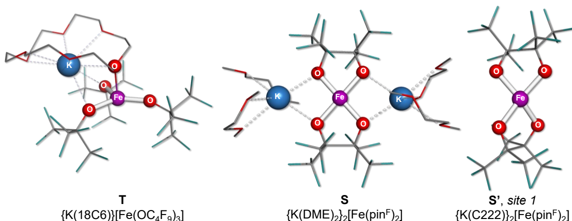
Figure 1. SCXRD-determined structures of T , {K(18C6)}[Fe(OC 4 F 9 ) 3 ] ( left ), S , {K(DME) 2 } 2 [Fe(pin F ) 2 ] ( middle ), and site 1 of S' , {K(C222)} 2 [Fe(pin F ) 2 ] without cations. Hydrogen atoms were omitted, fluorine atoms shown in teal, and carbon atoms in gray. The S , S' and T labels highlight the square ( S/S' ) and trigonal ( T ) geometries of the corresponding iron sites.
