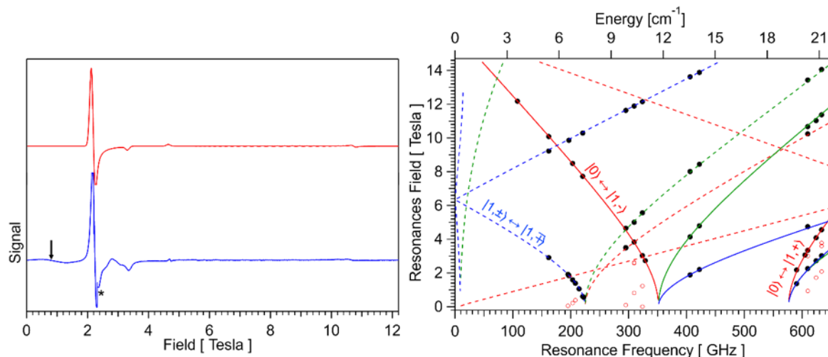
Figure 2. Left: Experimental ( blue ) HFEPR spectrum recorded for S at 20 K using a microwave frequency of 609.6 GHz and theoretical curve ( red ) obtained using the parameters listed in Table 1. The black arrow highlights a resonance not accounted for in our analysis and the feature marked by the asterisk is an instrumental artifact. Right: A field vs frequency plot in which black dots indicate the resonant fields and frequencies of the experimental resonances used to derive the spin Hamiltonian parameters of S . The red circles indicate the resonances not included in our analysis. The solid curves account for the theoretical dependencies of the ground state resonances and the dashed curves of the excited state resonances. The red, blue, and green colors account for the z , y , and x molecular directions, respectively.
