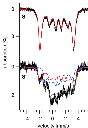
Figure 8. Comparison of the 4 K, 6 T Mössbauer spectra recorded for S ( top ) and S' ( bottom ). The theoretical spectra of S' were obtained using the parameters listed in Tables 1-3 for site a ( red ) and site b ( blue ). The complete set of field-dependent spectra acquired for S' are presented in Figure S14-S15.
