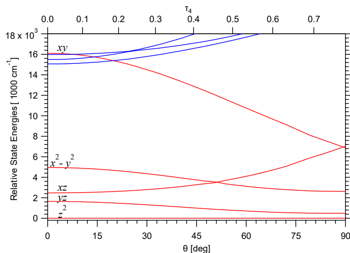
Figure 11. Relative energies of the five quintet states, shown in red, and of the three lowest triplet states, represented in blue, predicted by CASSCF(5,6) calculations which considered all five quintet and all 35 triplet states performed on the geometry optimized structures derived from the BP86/def2-TZVPP relaxed scan along \theta for \delta\lambda\text{-}[\text{Fe}(\text{pinF})_2]^{2-} . The labels of the quintet states refer to the states of the approximately square planar geometry ( C_{2h} ), at \theta = 0^\circ .
