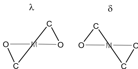
Scheme 2. Five membered ring with \lambda and \delta chelate ring conformations experimentally observed for the [Fe(pin F ) 2 ] 2- anions.
