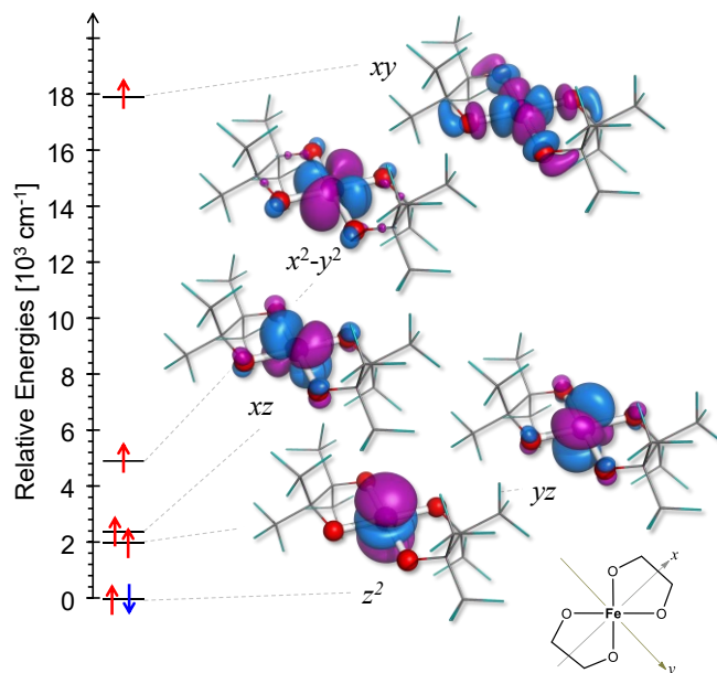
Figure 12. Crystal field splitting diagram inferred from a CASSCF(5,6)/def2-TZVPP calculation which considered 5 quintet and 35 triplet states performed on [\text{Fe}(\text{pin}^{\text{F}})_2]^{2-} anion, derived from the X-ray structure of S .
