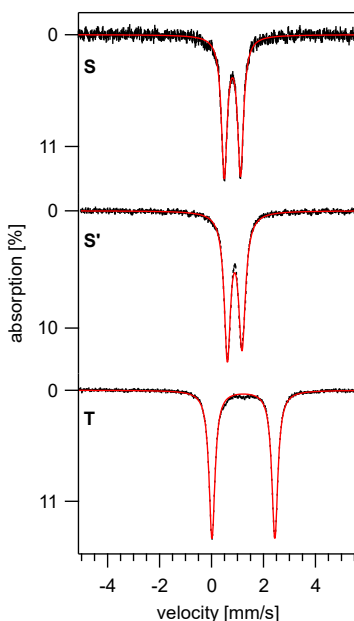
Figure 6. Zero field Mössbauer spectra recorded at 4 K for S ( top ), S' ( middle ) and T ( bottom ). The solid red lines are theoretical spectra obtained using a Lorentzian lineshape with a linewidth \Gamma = 0.27 mm/s for S , \Gamma = 0.29/0.32 mm/s for S' , and \Gamma = 0.28 mm/s for T and the parameters listed in Table 2.
