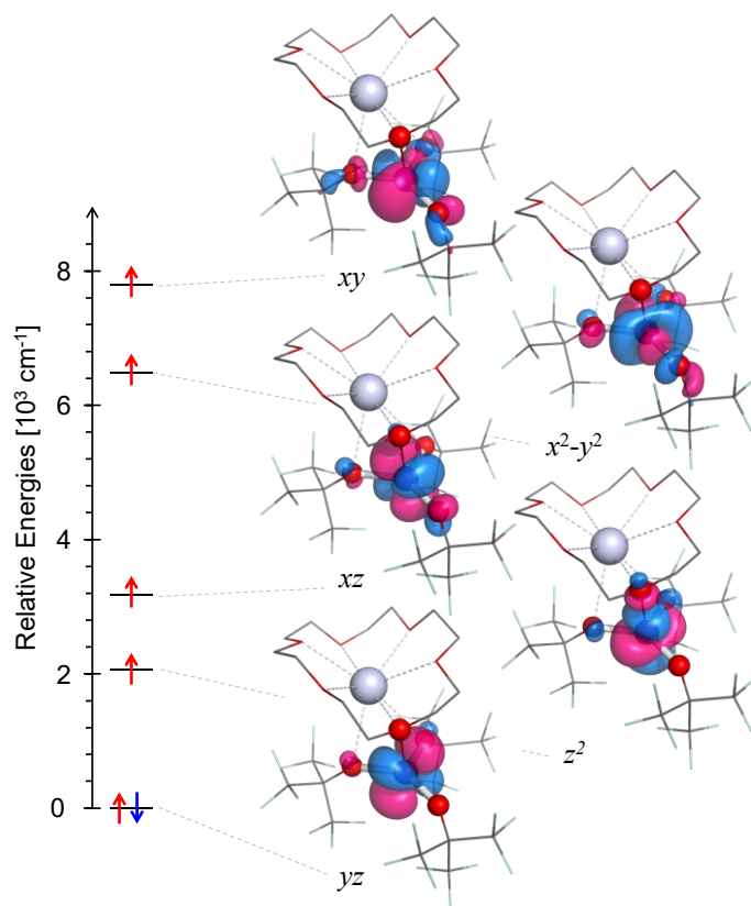
Figure 14. Crystal field splitting diagram inferred from a CASSCF(5,6)/def2-TZVPP calculation which considered 5 quintet and 35 triplet states performed on the unabridged X-ray structure of T .
