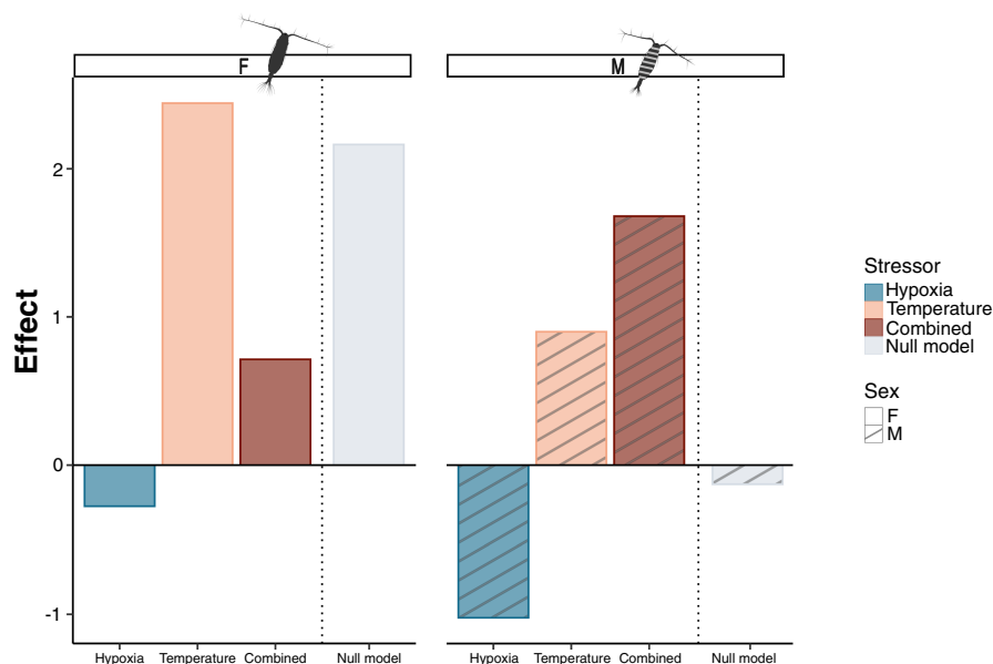
FIGURE 5 | Multistressor models showing antagonistic and synergistic effects of combined hypoxia and a MHW condition on A. tonsa 's females (left panel) and males' (right panel) CT_{max} . The bar plot represents the single effect of hypoxia (H, in blue) and temperature (MHW, in orange) and the combined effect of both stressors (HMHW, in red) in comparison with the calculated additive null model (H + MHW, in light grey).
