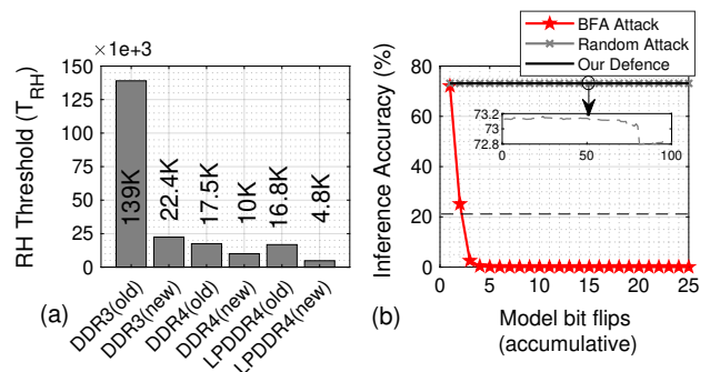
Figure 1: (a) RowHammer thresholds [21], (b) Targeted vs. random bit flipping for an 8-bit ResNet-34 on ImageNet and DNN-Defender 's performance.
