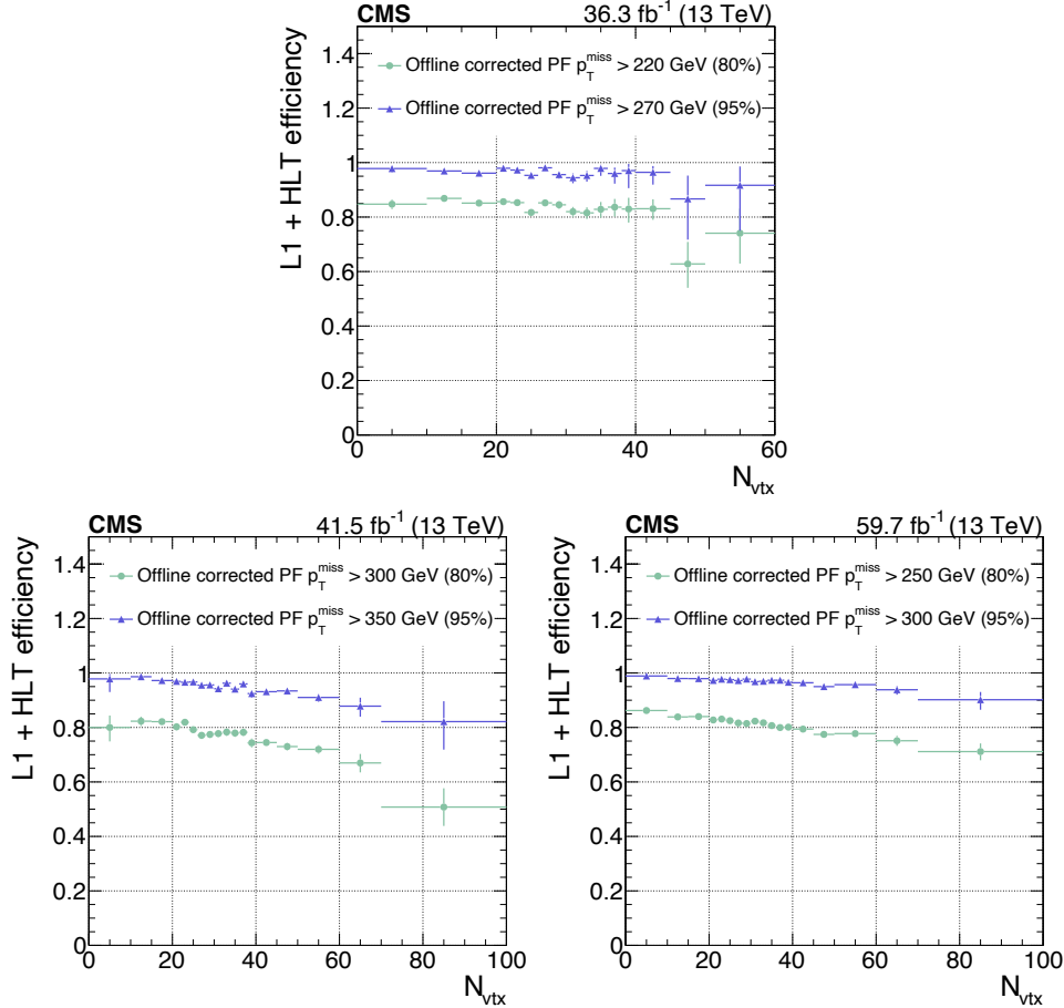
Figure 18. Event selection efficiencies as a function of N_{\text{vtx}} for fixed L1+HLT efficiency values of 80 and 95% of the unscaled p_T^{\text{miss}} triggers with the lowest p_T^{\text{miss}} thresholds in 2016 (upper), 2017 (lower left), and 2018 (lower right). The PU is considerably lower in 2016, which allowed to lower thresholds for all triggers involving jets and p_T^{\text{miss}} . The vertical bars on the markers represent statistical uncertainties.
