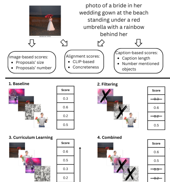
Figure 1. Top: we extract two image-caption alignment difficulty scores, two caption-based scores, and two image-based scores. Bottom: we train WSOD models by (1) randomly sampling images (baseline), (2) filtering out low-scoring samples, (3) using curriculum learning to sort images and sample high-scoring ones before low-scoring ones, and (4) combining (2) and (3) by applying curriculum learning to the top-scoring images only.
