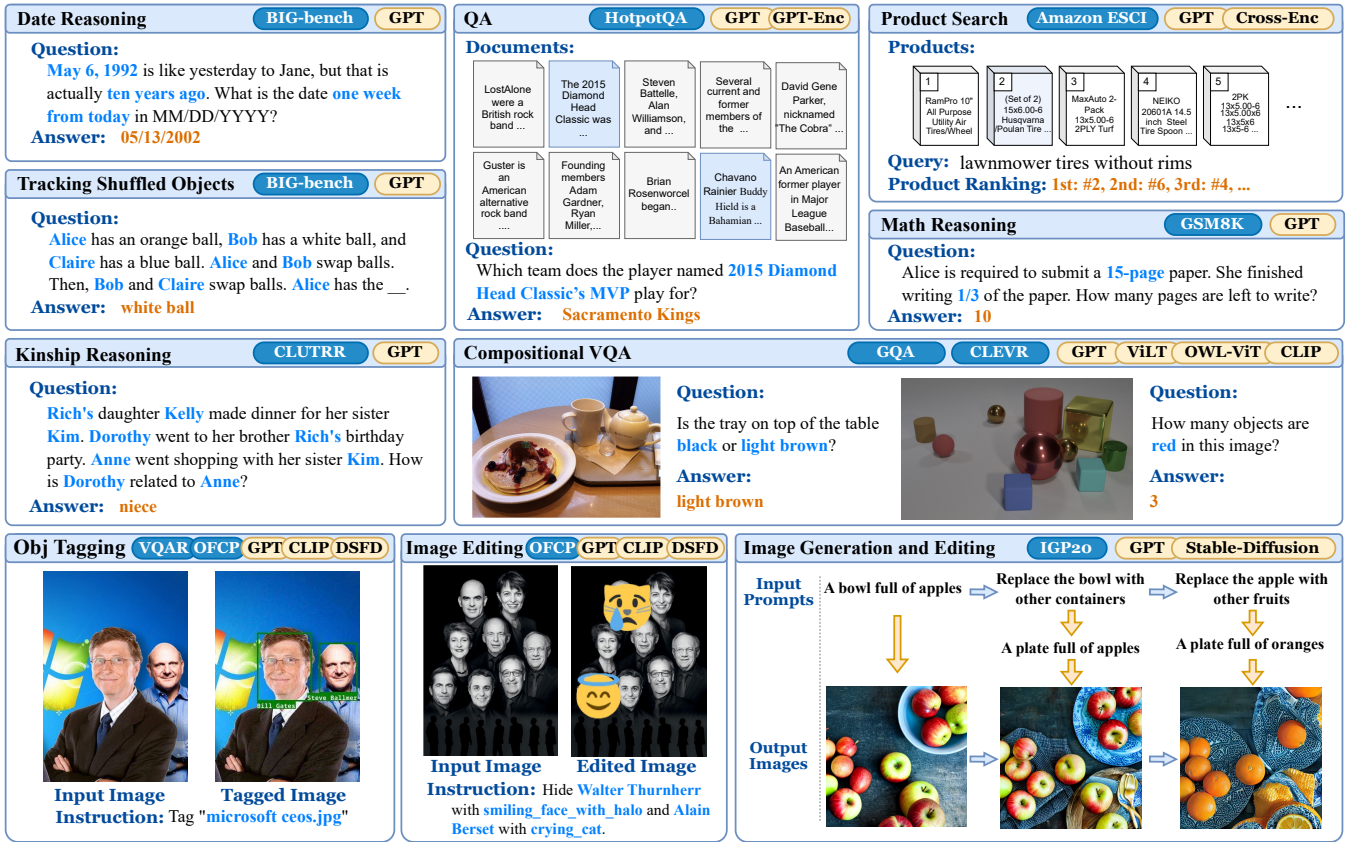
Figure 3: Benchmark tasks. The top of each box lists the dataset(s) and the foundation models used in our solutions.
