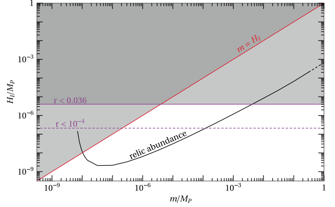
FIG. 3. Values of H_I and m that yield the observed DM relic abundance [69,70] in the case where freeze-in production from elementary gauge bosons dominates over CFT production (black line). We assume all of the SM gauge bosons are elementary, are reheated at the end of inflation, and couple universally to the DM with \kappa_v = 1 . We fix m/\Lambda = 0.1 . The bounds are the same as in Fig. 1.
