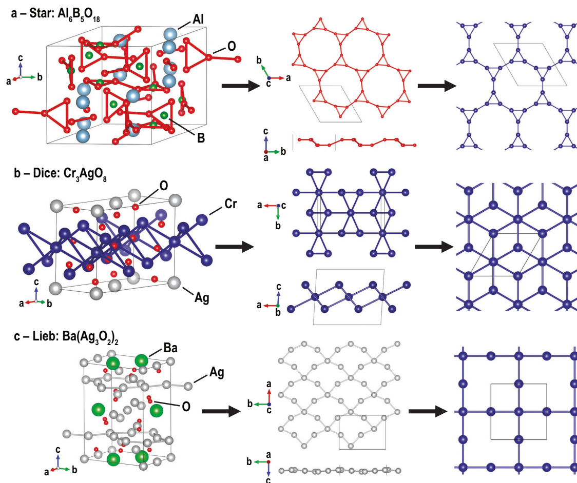
Fig. 5 | Distorted lattices and higher symmetry flat band lattices. a (left) Structure of \text{Al}_6\text{B}_5\text{O}_{18} , (center) its isolated oxygen star lattice, and (right) the topologically equivalent higher symmetry counterpart. b Structure of \text{Cr}_3\text{AgO}_8 , its isolated
