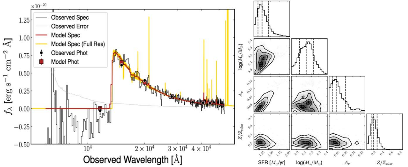
Figure 4. Stellar population synthesis modeling with Bagpipes. The left panel shows the observed galaxy SED and spectrum (black, showing only JWST photometry) after the application of the polynomial calibration with 1\sigma errors (assuming an error floor of 5%) and the median model (red). Additionally, the median model is shown at the full resolution (gold), highlighting the predicted emission features that are washed out by the instrumental resolution. In the right panel, we show the covariant posteriors for a number of key measured parameters after accounting for the magnification of the source.
