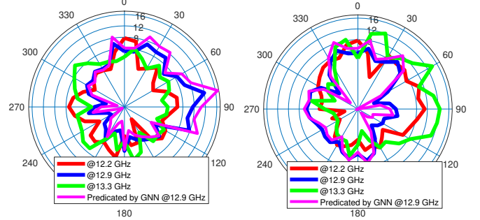
Fig. 4. RPs for antenna-2 at \phi = 0 (left), \phi = 90^\circ (right).
