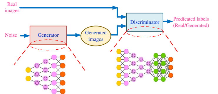
Fig. 1. Typical diagram of GAN structure.
