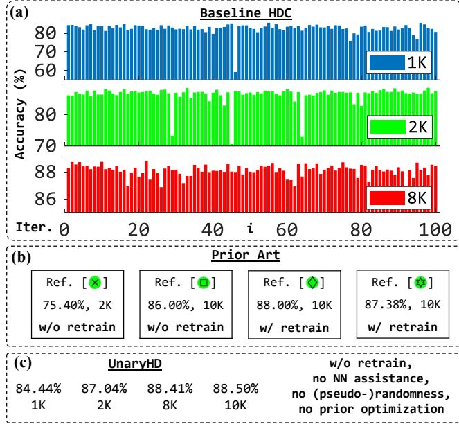
Fig. 6. Different accuracy monitoring of HDC designs. Accuracy fluctuations at each iteration of the baseline design with (pseudo-)randomness (a), MNIST dataset accuracy from prior HDC works; Ref.s [4], [19], [28], [9], [29] (b), and uHD (c).
