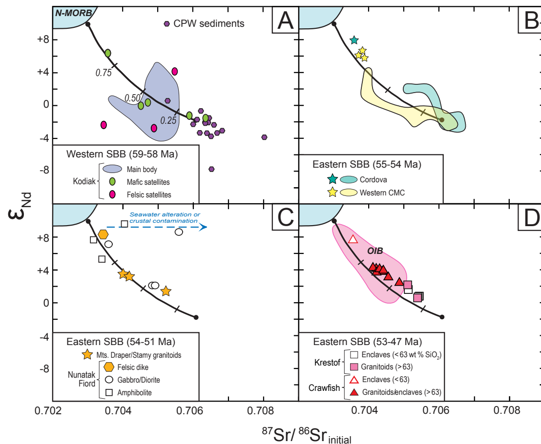
Figure 10. \epsilon_{\text{Nd}} vs. ^{87}\text{Sr}/^{86}\text{Sr}_{\text{initial}} diagrams for whole-rock samples from this study and other previously published Sr-Nd isotopic data sets for Sanak-Baranof belt (SBB) intrusive rocks. Mixing curves (after Harris et al., 1996) between normal mid-ocean-ridge basalt (N-MORB) and an average Chugach–Prince William (CPW) sedimentary composition are shown in each panel. The numbers next to the tick marks in panel A denote the weight fraction of MORB that was added to sediment in each mixing model. (A) Kodiak batholith samples (data from Ayuso et al., 2009). Also shown are compositions of CPW sedimentary rocks (whole-rock compositions from Farmer et al., 1993, plus one sample from Harris et al., 1996). (B) Intrusive rocks from the Cordova area (Barker et al., 1992) and western Chugach metamorphic complex (CMC; Sisson et al., 2003b). Stars denote late-stage intrusions. (C) Nunatak Fiord and Mount Draper/Stamny samples (Sisson et al., 2003b). Blue dashed arrow is a trend associated with seawater contamination and/or crustal assimilation (Sisson et al., 2003b). (D) Crawfish Inlet and Krestof Island samples (this study). The pink field represents oceanic-island basalts (OIB) after Zindler and Hart (1986), Hofmann (1988, 1997), Sun and McDonough (1989), and Salters and Stracke (2004).
