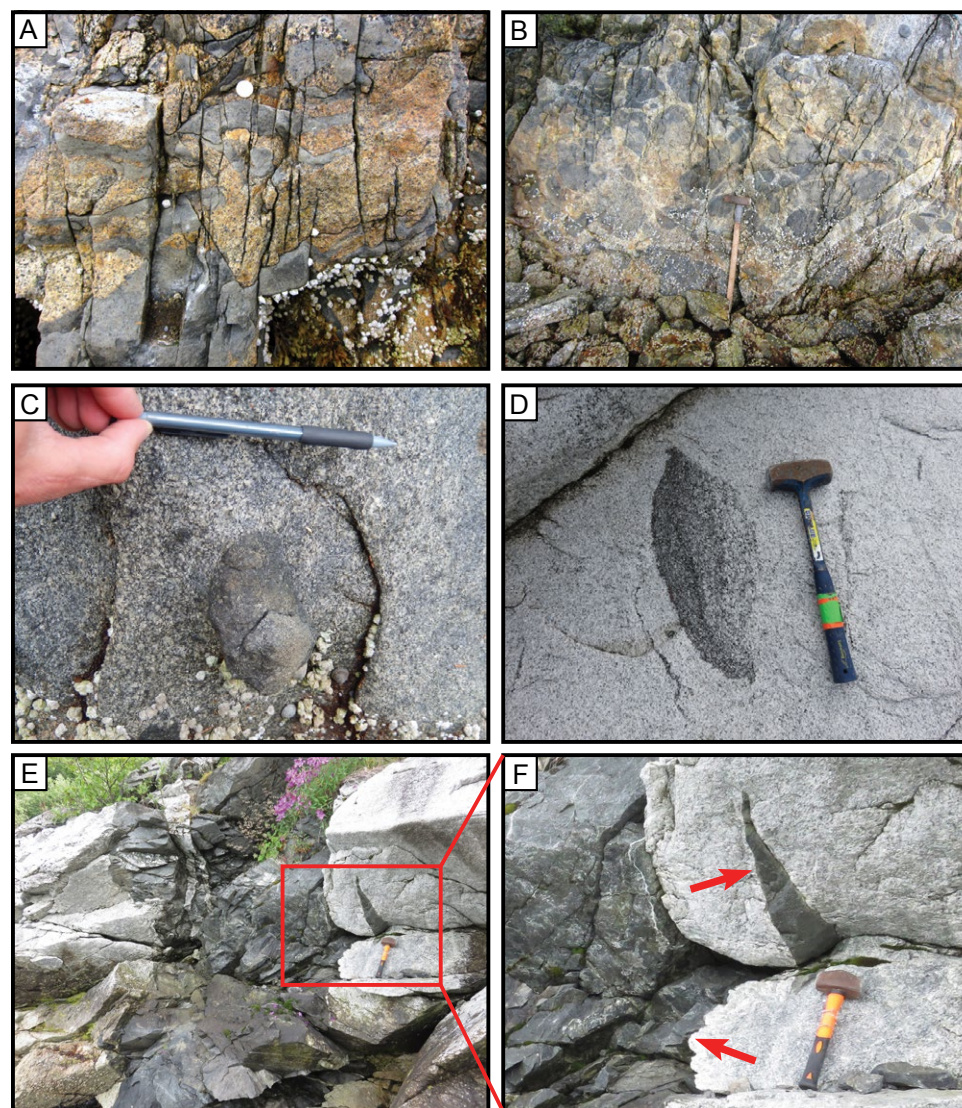
Figure 4. Field photos of select plutons from the eastern Sanak-Baranof belt (Boundary block and Baranof Island area). (A) Mafic enclave swarm in the Crawfish Inlet pluton. Note the cuscate-lobate boundaries between the mafic and felsic rocks; quarter (~2.4 cm diameter) for scale. (B) Mafic enclave swarm emplaced in the Krestof pluton; note the rock hammer (~0.4 m in length) for scale. (C) Typical Krestof Island magmatic enclave exhibiting roundish shape, higher color index, and aphanitic texture relative to its host. (D) Mafic enclave in the Mount Draper host granite. (E) Mutually crosscutting relationships between a mafic dike (sample RF 16–30B) and the Mount Draper pluton. (F) Zoomed image of the panel E inset. Upper red arrow shows an isolated xenolith of the mafic dike in the host granite, and the lower arrow highlights cuscate-lobate texture between the dike and host granite, which indicates a comagmatic relationship.
