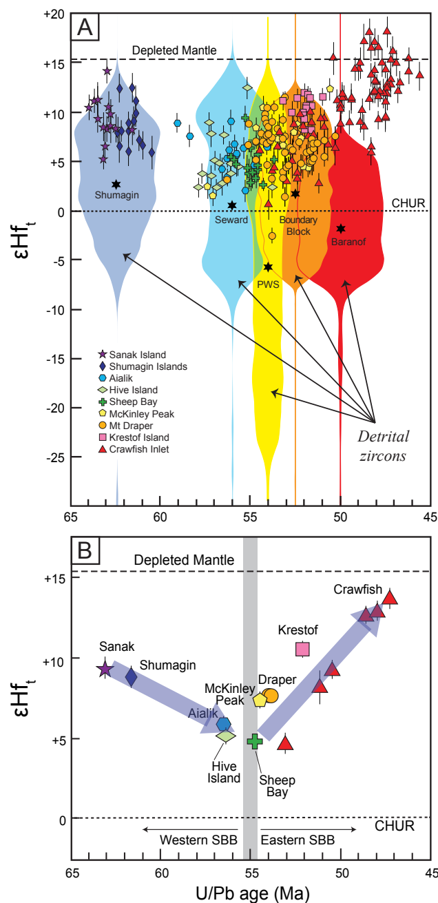
Figure 11. (A) \epsilon Hf_t values of magmatic zircon from the Sanak-Baranof belt plutons (plotted as symbols) compared with \epsilon Hf_{50Ma} values for detrital zircon from various Chugach–Prince William turbidite groups (plotted as shaded areas of various colors). Color shaded fields are bubble plots that were constructed from probability density plots of the detrital zircon \epsilon Hf_{50Ma} data (see Methods and Table S3 [text footnote 2]) and are centered near the U–Pb ages of the intruding plutons. Black stars are the average \epsilon Hf_{50Ma} values of the detrital zircons. Vertical error bars are \pm 1\sigma . CHUR—chondritic uniform reservoir; PWS—Prince William Sound. (B) Weighted means of the \epsilon Hf_t data from the Sanak-Baranof belt (SBB) plutons. Vertical error bars are \pm 2\sigma . Blue arrows highlight the V-shaped time-transgressive trend in \epsilon Hf_t values for the Sanak-Baranof belt plutons through time.
