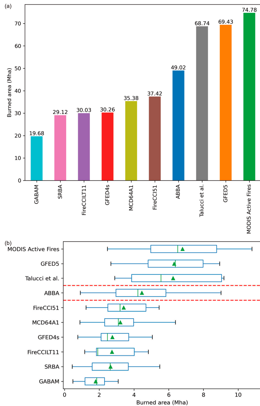
Figure 4. Total BA (a) and box and whisker plot (b) for each dataset for the analysis period (2006–2016) in central/northern Siberia. The whiskers extend to 1.5 \times Inter-Quartile Range. The mean of each dataset is given as the green triangle. “Talucci et al.” refers to the Talucci et al. (2022) fire perimeter product [63].
