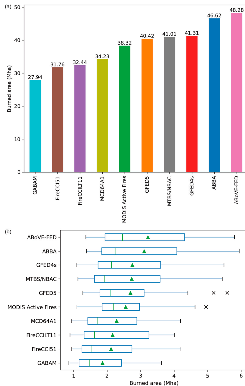
Figure 2. Total BA (a) and box and whisker plot (b) for each dataset for the analysis period (2002–2016) in North America. The whiskers extend to 1.5 \times Inter-Quartile Range. The mean of each dataset is given as the green triangle.
