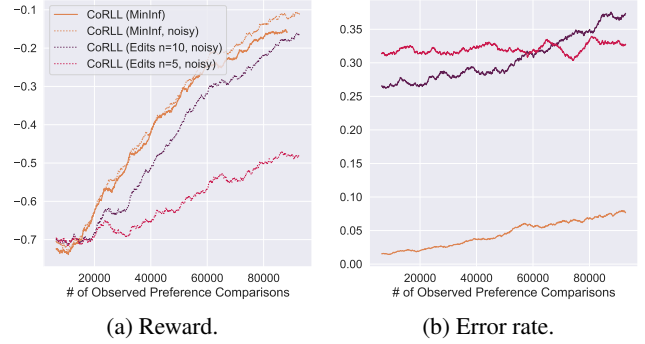
Figure 4. Summarization task with noisy feedback. Reward and error rates are a rolling average over 100.
