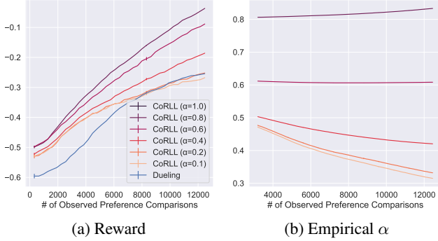
Figure 9. Experimental results for varying feedback quality on IMDB. Coactive (CoRLL MinInf) in purple-orange, duelling in blue.
