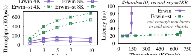
Figure 13. Scalable Throughput with Erwin-st.
