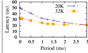
Figure 10. Periodicity vs Latency.
