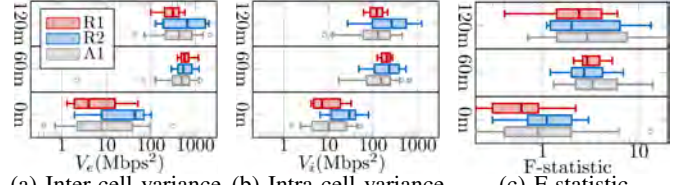
Fig. 9: Performance diversity of 5G cells over R1, R2, and A1.
