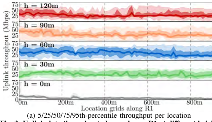
Fig. 3: Uplink data throughput observed over R1 at different heights ( h = 0\text{m}, 30\text{m}, 60\text{m}, 90\text{m}, \text{and } 120\text{m} ).
