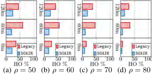
Fig. 19: HO ratio without selecting good cells.
