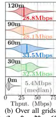
Fig. 3: Uplink data throughput observed over R1 at different heights ( h = 0\text{m}, 30\text{m}, 60\text{m}, 90\text{m}, \text{and } 120\text{m} ).
