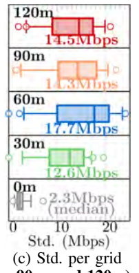
Fig. 3: Uplink data throughput observed over R1 at different heights ( h = 0\text{m}, 30\text{m}, 60\text{m}, 90\text{m}, \text{and } 120\text{m} ).
