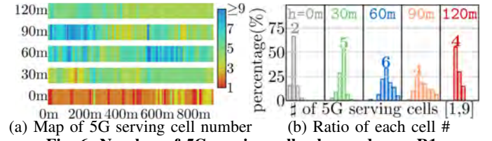
Fig. 6: Number of 5G serving cells observed over R1.
