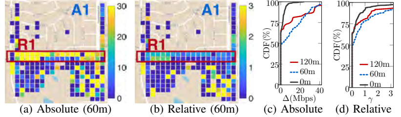
Fig. 20: Absolute gain \Delta and relative gain \gamma with 5GAIR in A1.
