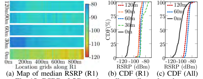
Fig. 15: RSRP of 5G serving cells at all test locations.
