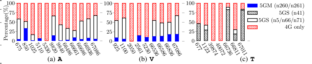
Fig. 16: Breakdown of SCell RATs per 4G PCell channel.
