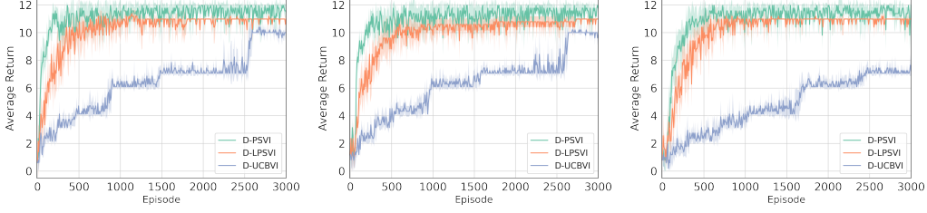
Figure 1: Left:(a) Multinomial delay with delay categories \{10, 20, 30\} . (b) Poisson delay with rate \mathbb{E}[\tau] = 50 . (c) Long-tail Pareto delay with shape 1.0, scale 500. Results are reported over 10 experiments. Delayed-PSVI and Delayed-LPSVI demonstrate robust performance under both well-behaved and long-tail delays.
