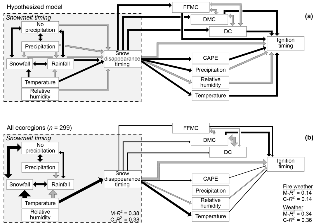
Figure 6. Piecewise structural equation model (pSEM) of the hypothesized snow disappearance and ignition timing model (a) and its fit for all ecoregions (b). The influences of fire weather and weather on ignition timing were modeled separately. Gray arrows represent positive effects and black arrows indicate negative effects. The single-headed arrows show significant direction of causal relationships, while double-headed arrows represent significant non-causal relationships ( p < 0.1 ). All arrows are scaled to their respective effect size (Table S11). Marginal R^2 ( M-R^2 ) indicates the variation solely explained by the fixed effects, and conditional R^2 ( C-R^2 ) represents the variation explained by both the fixed and random effects.
