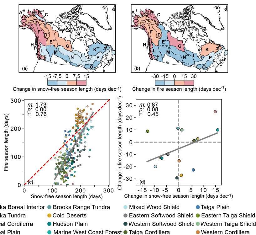
Figure 4. Changes in the snow-free season length (d decade -1 ) for all ecoregions (A–P) between 2001 and 2019 (a) and the changes in the fire season length (d decade -1 ) per ecoregion (A–P) between 2001 and 2019 (b) (Table S10). Letters correspond to the respective ecoregion names (Fig. 2), and significant relationships are indicated by * ( p < 0.1 ) and ** ( p < 0.05 ). The relationship between the annual absolute length of the snow-free season from the MODIS product (days) and annual length of the fire season for all ecoregions (c), as well as the ecoregional trends in snow-free and fire season length (d decade -1 ) (d).
