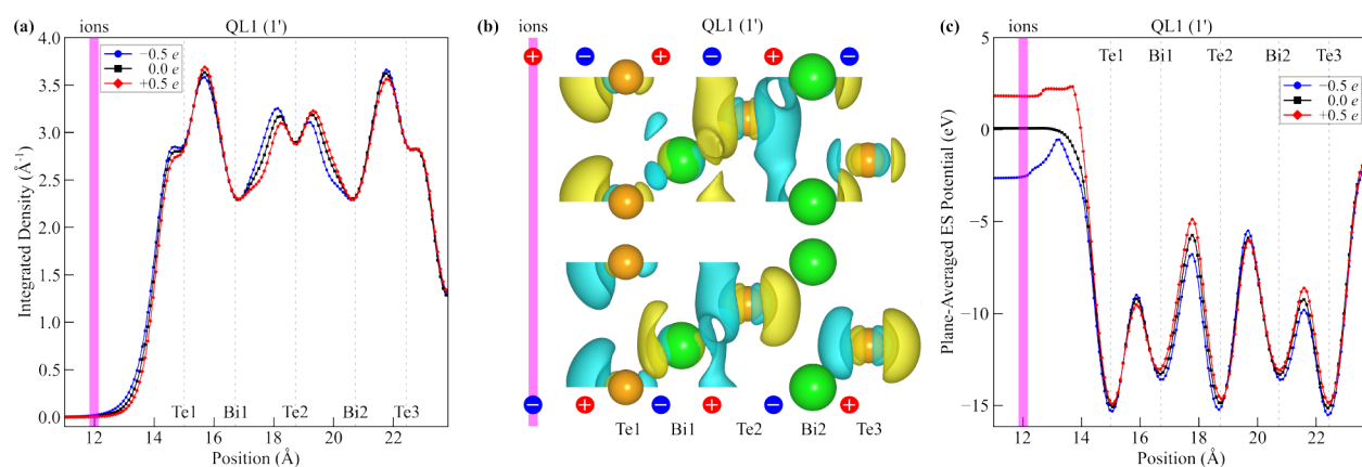
Figure 3. (a) Integrated electron density over the xy -plane at various sampled positions along the z -axis (perpendicular to the surface) of the \text{Bi}_2\text{Te}_3 slab. The plot focuses on QL1 (1') where apparent electron density fluctuations occur in response to surface charging (black for 0 e , red and blue for +0.5 e and -0.5 e , respectively). The gray dotted lines denote the ionic positions, and the magenta bar marks the peak of the integrated counter-charge density, which is \sim 3 Å away from the surface. (b) Visualization of the change in electron density in a three-dimensional real space grid. Relative to the charge-neutral slab, regions gaining electrons are shown in yellow, while regions losing electrons are in cyan. Induced dipoles are inferred from these density fluctuations and indicated by blue and red circles. (c) Plane-averaged electrostatic (ES) potential within QL1 (1') along the z -axis for the same three charging states in (a).
