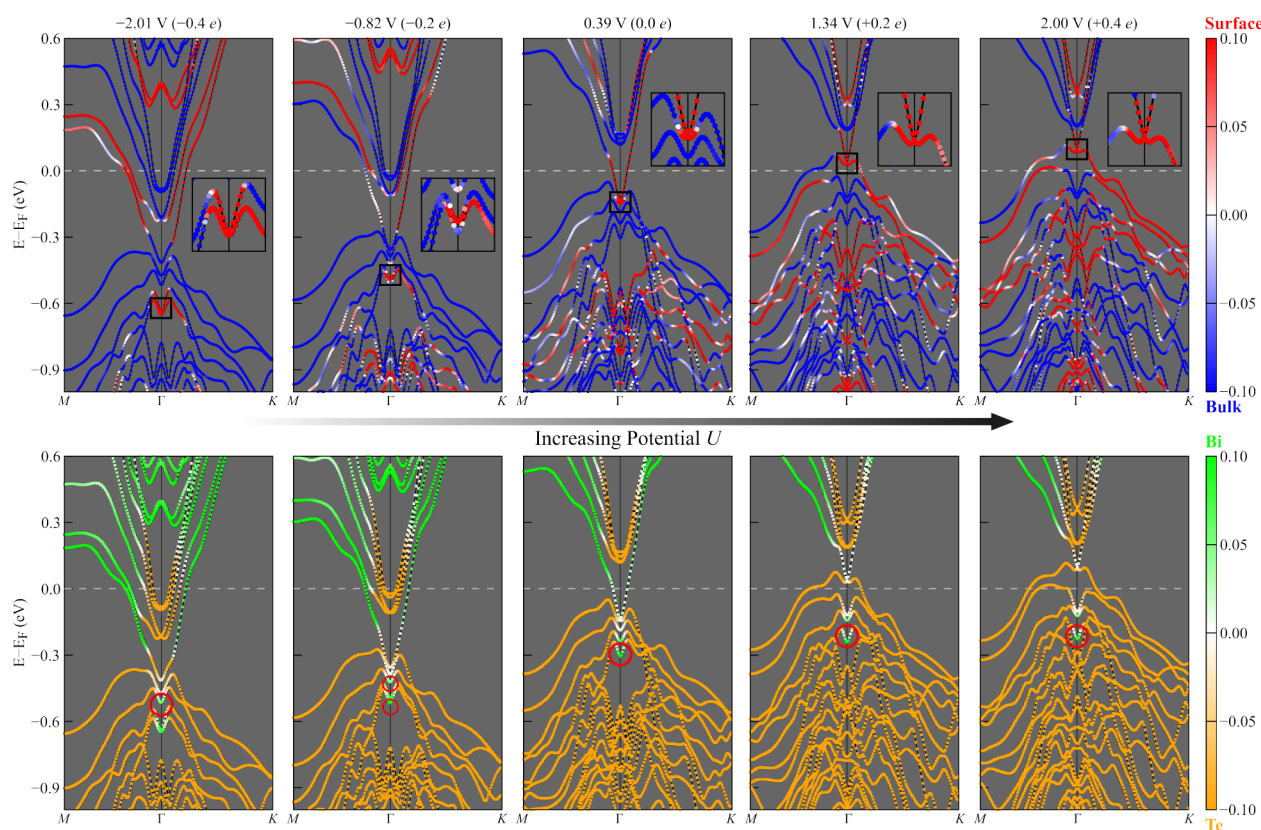
Figure 2. Projected band structures of the \text{Bi}_2\text{Te}_3 slab under various electrode potentials. In each panel, the electronic states are color-coded to reflect their predominant orbital contributions. Upper panels: electronic states depicted in red are primarily derived from the surface, while those in blue are dominated by the bulk. Lower panels: electronic states depicted in green originate primarily from the Bi atoms, while those in orange are Te-dominated. The black squares in the upper panels track the evolution of the surface Dirac point, which is further highlighted in the inset. The red circles in the lower panels highlight the electronic states that exhibit band inversion around the \Gamma point.
