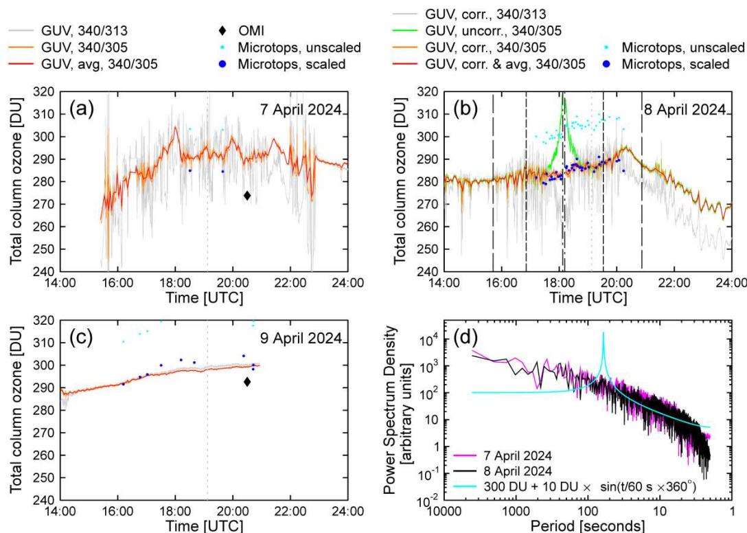
Figure 9: Measurements of TCO at Mazatlán on (a) 7 April 2024, (b) 8 April 2024, (c) and 9 April 2024. \text{TCO}_{340/313} and \text{TCO}_{340/305} measurements at 1 Hz are shown in gray and orange, respectively. The red line shows 90 second moving averages of TCO derived from \text{TCO}_{340/305} . Microtops measurements are biased high (cyan circles). Data scaled down by 6.5 % are also shown (blue) for ease of comparison with GUV data. OMI measurements are only available on 7 and 9 April 2024. All data were filtered for SZAs smaller than 75^\circ . The vertical “very long-dashed” vertical lines (before 16:00 and at about 21:00) indicate the times when the shadow of the Moon either first hit the Earth (over the Pacific) or leaves the Earth (over Greenland). 1 st and 4 th contact at Mazatlán are indicated by dashed lines, and the 2 nd and 3 rd contact are indicated by dashed-dotted lines. Panel (d) shows the power spectrum density of \text{TCO}_{340/305} between 18:14:00 and 19:22:16 on 7 and 8 April 2024. The PSD for a hypothetical scenario where TCO oscillates with an amplitude of 10 DU and a period of 60 s about a constant value of 300 DU is also shown (cyan line).
