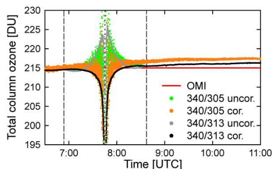
Figure 17: GUV measurements of TCO at Union Glacier on 4 December 2021. Uncorrected and LD-corrected \text{TCO}_{340/305} data are shown in green and orange, respectively. Similar data calculated for \text{TCO}_{340/313} are shown in grey and black. The average of OMI measurement for this day is indicated by a horizontal red line. Long-dashed lines indicate the 1 st and 4 th contact. The 3 rd and 4 th contact are indicated by dashed-dotted lines.
