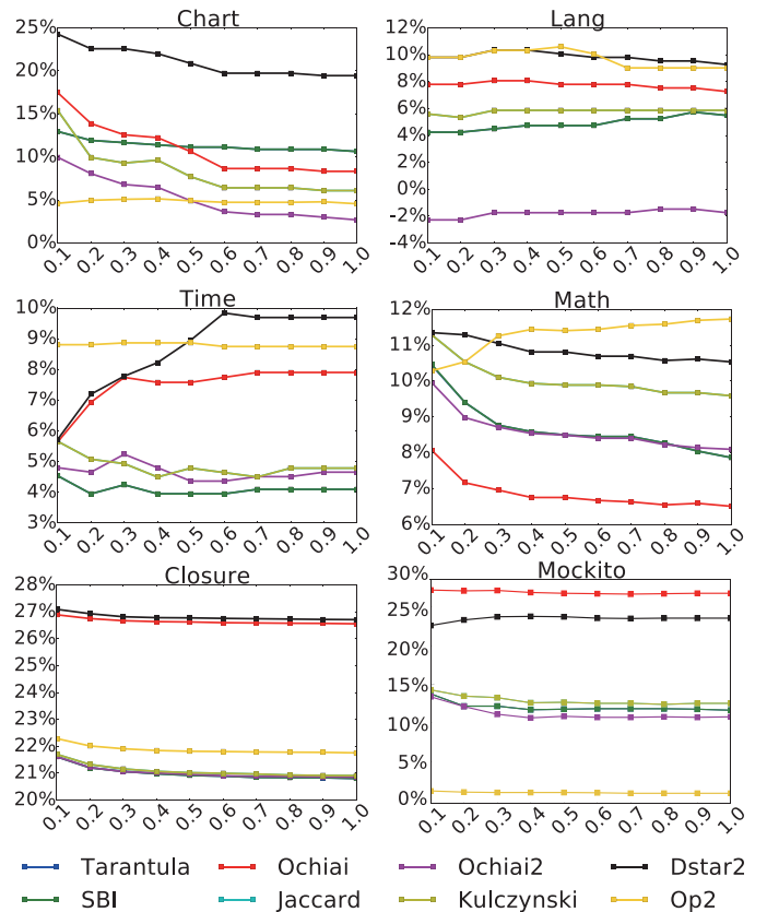
Fig. 7. Impact of damping factor.
