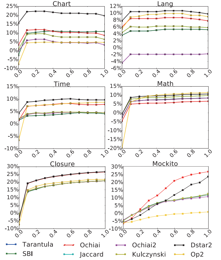
Fig. 9. Impact of return weight.
