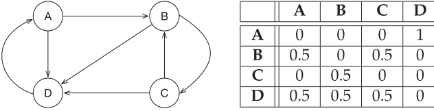
Fig. 1. A small network and its transition matrix.
