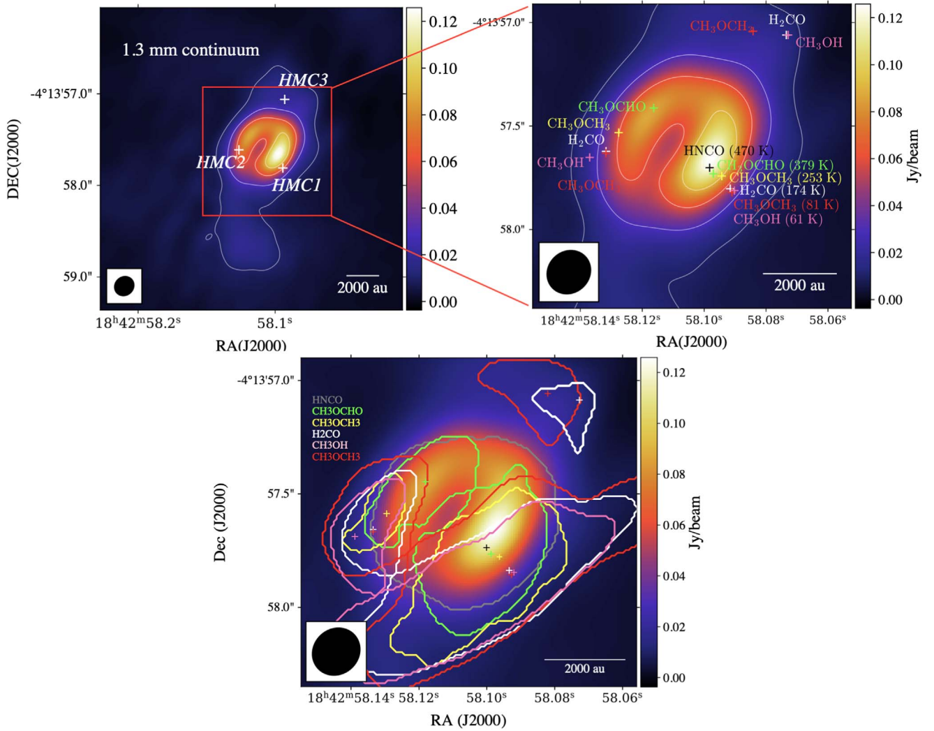
Figure 1. (a) Top left panel: continuum map of G28.2 obtained with ALMA at 230 GHz. Contour levels start at 3\sigma ( 1\sigma = 1 \text{ mJy beam}^{-1} ) and steps are in 3\sigma . The ellipse at the bottom-left corner of the image shows the synthesized beam ( 0''.22 \times 0''.20 ) with PA = -47^\circ . Three white crosses represent the positions of HMC1, HMC2, and HMC3. (b) Top right panel: zoom-in of the central region, including locations of various molecular line emission peaks and associated upper-state energies. Note the implied temperature gradients along directions pointing away from the main millimeter continuum peak. (c) Bottom panel: same as (b), but now showing contours of different dendrogram leaves of several identified species (see the text).
