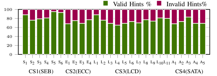
Fig. 20: Percentage of valid and invalid hints generated by HIVE framework for different scenarios of four case studies. Here S1 to S6, E1 to E4, L1 to L11 and A1 to A5 denotes scenarios corresponding case studies CS1, CS2, CS3, and CS4.
