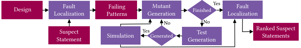
Fig. 18. Fault localization using directed tests [29]
