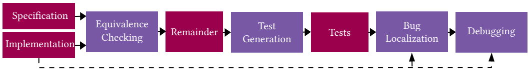
Fig. 19. Directed test generation for faster bug localization [36]
