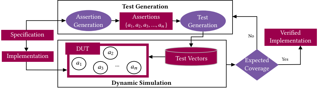
Fig. 16. Overview of directed test generation during assertion-based validation.
