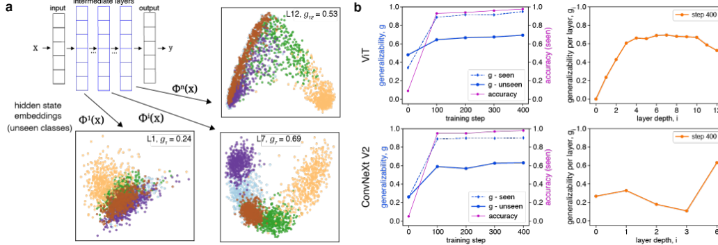
Figure 1: Generalizability and accuracy are loosely coupled. (a) An overview of our method of assessing generalizability through out-of-sample embeddings using intermediate layers, visualized using PCA. Embeddings from different hidden states of the Vision Transformer (ViT) produce widely varying results. Color labels indicate ground truth: clustered unseen classes indicate better generalization ( g ). (b) Results for ViT (top) and ConvNeXtV2 (bottom). Across epochs, test-set accuracy monotonically increases while generalizability may plateau or even decrease (left). Across layers, there are no predictable trends (right). For additional results, see Appendix.
