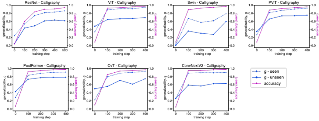
Figure 4: Generalization across fine-tuning epochs for all studied networks. We plot g_{s-n} and test-set accuracy (using seen classes) for reference. Notice how g_{s-n} is higher for all networks, as expected. This demonstrates that our g metric is able to capture the ability of the networks to generalize to unseen classes.
