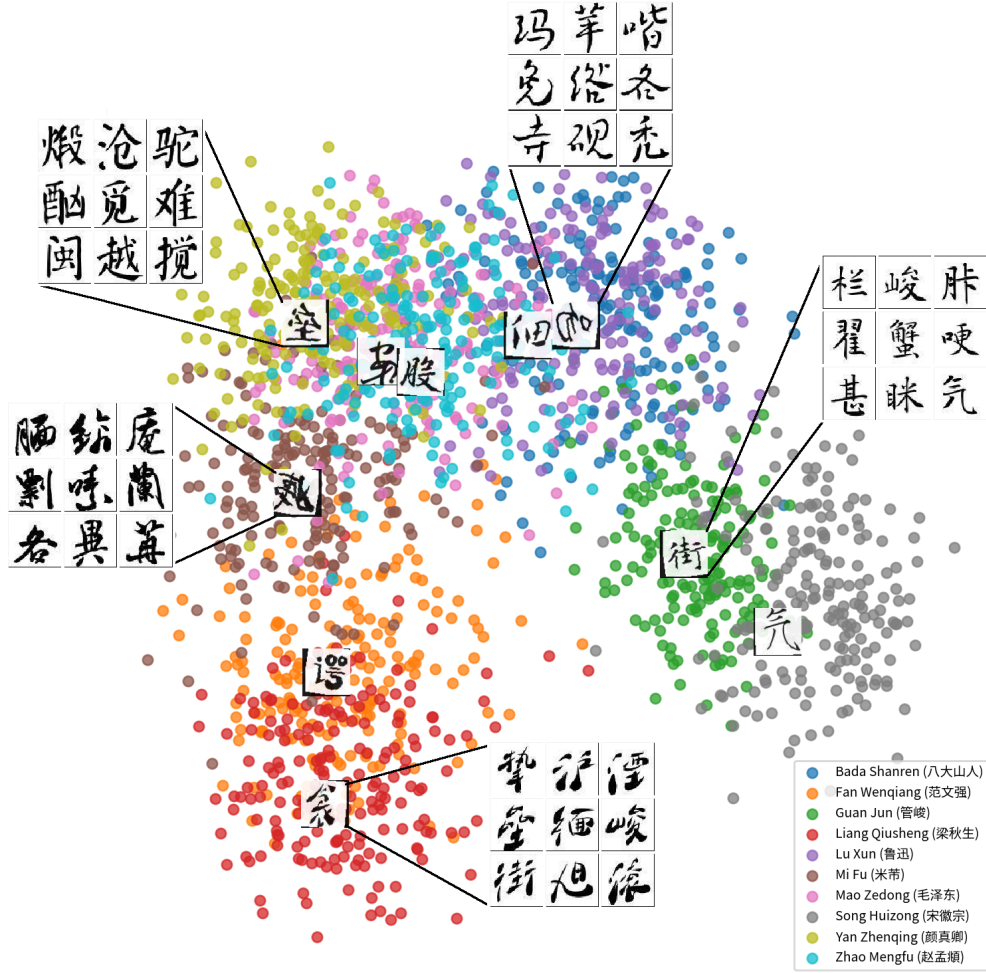
Figure 3: Embedding of 10 calligraphers (including in-sample and out-of-sample) obtained via ResNet and visualized using PC , with representative character images for each of the ground-truth clusters shown. The images were chosen by computing the centroid of each cluster and selecting those corresponding to the 10 nearest points.
