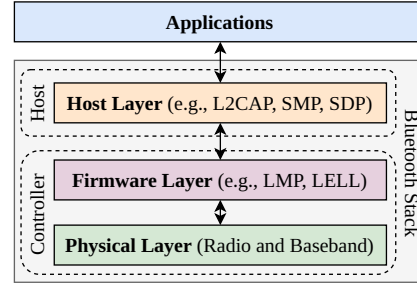
Figure 1: Layers of a Bluetooth stack.
