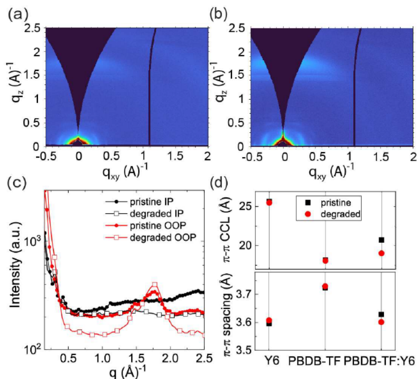
Figure 5. (a), (b) GIWAXS diffraction patterns of pristine and degraded PBDB-TF:Y6 blends, respectively. (c) Line cuts along in-plane (IP) and out-of-plane (OOP) directions for pristine and degraded blend films. (d) \pi - \pi crystal coherence length (CCL) and \pi - \pi spacings for pure Y6 , pure PBDB-TF , and PBDB-TF:Y6 blend films before and after degradation.
