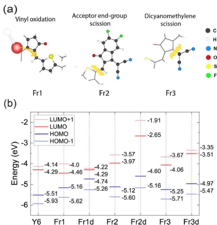
Figure 6. (a) Chemical structures of three types of possible single fragmentation products of a degraded Y6 molecule. Single (double) fragmentation via vinyl oxidation, acceptor end-group scission, and dicyanomethylene scission are labelled as Fr1, Fr2, and Fr3 (Fr1d, Fr2d, and Fr3d), respectively. The full chemical structures of all variations of the degraded Y6 molecules are shown in Supporting Fig. S18. (b) Energy levels of frontier molecular orbitals (HOMO-1, HOMO, LUMO, and LUMO+1) on pristine Y6 and degraded products after six kinds of degradation on Y6.
