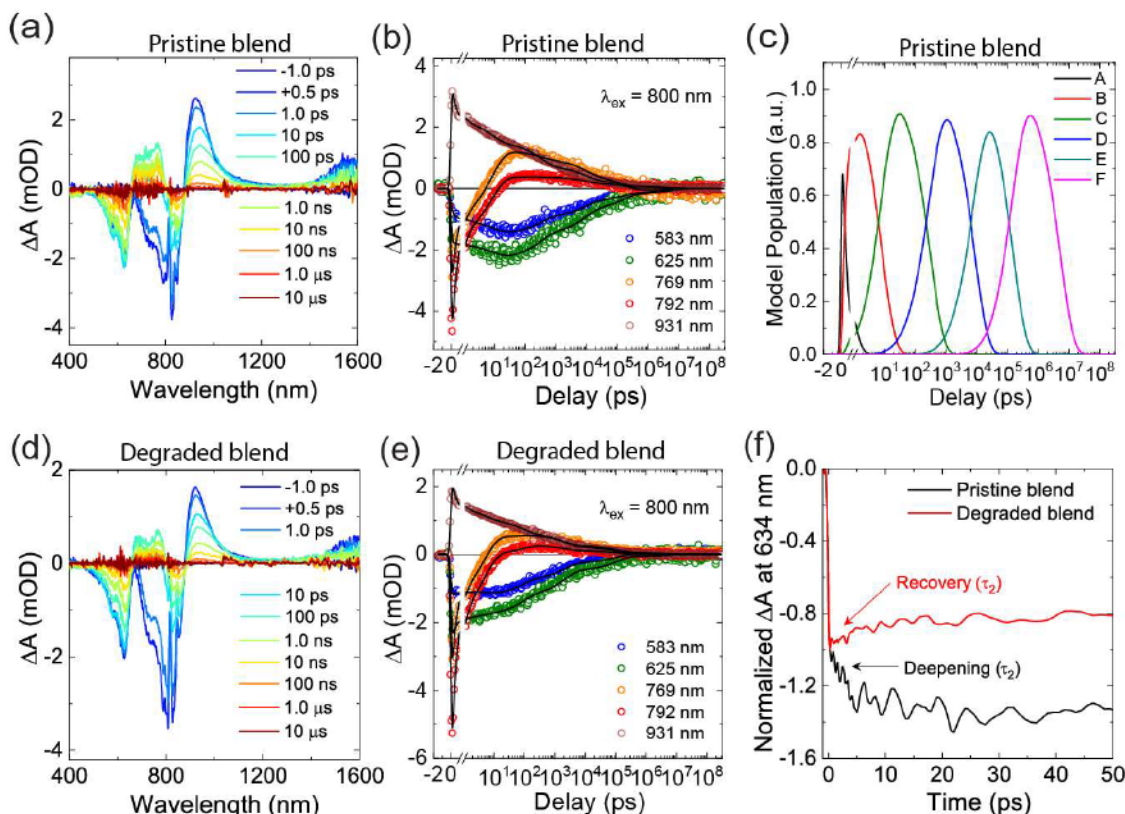
Figure 4. (a) Transient absorption (TA) spectra of a pristine PBDB-TF:Y6 blend film taken at different delay times when excited at 800 nm (20 mJ·cm -2 ). (b) Corresponding time-resolved differential absorption (ΔA) at indicated wavelengths (symbols). The solid lines show model fits from global analysis. (c) Model population dynamics of different species (A-F) in the pristine blend. (d), (e) TA spectra and time-resolved ΔA of the same PBDB-TF:Y6 blend film after degradation. (f) A comparison of bleach kinetics shows the deepening of the bleach in a degraded blend over a few picoseconds. The instrument response function is 300 fs.
