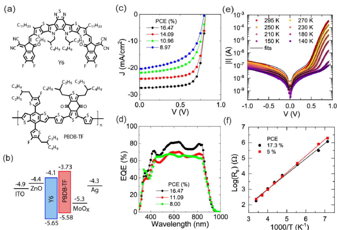
Figure 1. (a) Chemical structures of Y6 (top) and PBDB-TF (bottom) molecules. (b) Energy level alignment of the various layers in PBDB-TF:Y6 solar cells. (c) Current-density-voltage ( J - V ) characteristics of the solar cell at different PCE values during degradation. (d) External quantum efficiency (EQE) plot of the cell at different PCE values during degradation. (e) Dark J - V characteristics of a solar cell at varying temperatures from 140 – 295 K. Solid lines show fits to the Schottky diode equation. (f) Plot of \text{Log}(R_s) versus 1/T to extract E_s for pristine and degraded cells.
