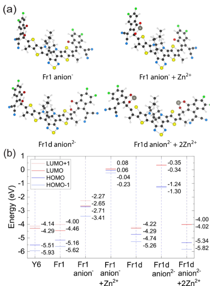
Figure 7. (a) Optimized molecular structures of the “ Fr1 anion - ” and “ Fr1d anion 2- ” that are singly and doubly charged fragments, respectively. To create an anion from Fr1 and Fr1d , a hydrogen atom was removed from the nitrogen atom within the dicyanomethylene group. Charges have been stabilized by \text{Zn}^{2+} in “ Fr1 anion - + Zn 2+ ” and “ Fr1d anion 2- + 2Zn 2+ ” fragments after additional removal of the hydrogen atom from the hydroxyl group. Charges have been stabilized by \text{Zn}^{2+} in “ Fr1 anion - + Zn 2+ ” and “ Fr1d anion 2- + 2Zn 2+ ” fragments. The atom color scheme is identical to that in Fig. 6a. \text{Zn}^{2+} is labeled as gray. (b) Frontier molecular orbital energy levels (HOMO-1, HOMO, LUMO, and LUMO+1) of pristine Y6 and degraded products Fr1 and Fr1d after each degradation on Y6 , depending on the charge state and the existence of \text{Zn}^{2+} . “ Fr1 anion - ” and “ Fr1d anion 2- ” have -1 and -2 as total charges, respectively, and all other molecules are charge neutral.
