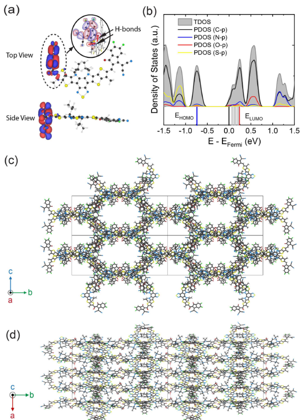
Figure 8. (a) LUMO of Fr1 molecule after vinyl oxidation. The inset shows the formation of hydrogen bonds around the hydroxyl group. The HOMO of Fr1 is shown in Supporting Fig. S20. (b) TDOS and PDOS ( p orbital of carbon, nitrogen, oxygen, and sulfur) of the Fr1 crystal structure. Energy levels of HOMO ( E_{\text{HOMO}} ), LUMO ( E_{\text{LUMO}} ), and trap energy levels are shown by blue, orange, and grey solid vertical lines below the x-axis. Energy spectra are smeared with a value of 50 meV. (c) and (d) Optimized crystal structure of Fr1 in top and side views, respectively, based on the original pristine Y6 crystal structure. The color scheme on each element is identical to that in Fig. 6a.
