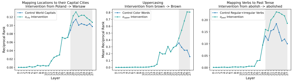
Figure 10: We use the same stimuli to extract \vec{o} vectors on GPT-J. Results are similar for the upercasing function, but only very weakly positive on the world capitals task.
