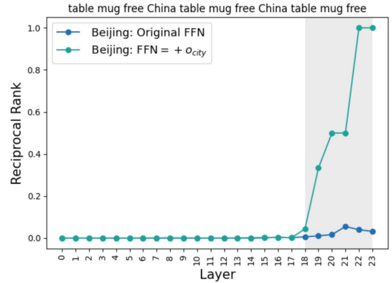
Figure 4: The gray area indicates layers with the FFN intervention. Even if the input context is nonsense (repeating pattern), when “China” is represented in the residual stream, the \vec{o}_{city} vector promotes the correct capital city.
