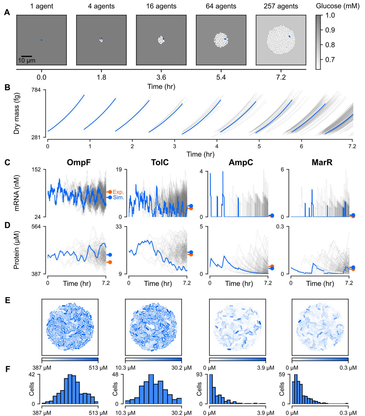
Fig 2. Spatio-temporal heterogeneity in baseline gene expression. (A) Snapshots of a simulated E. coli colony. The environmental glucose concentration is represented by varying shades of gray. The blue-colored cells are from a single representative cell lineage (cell 011000000 and its ancestors) and the time series data for that same lineage is also highlighted blue in panels B, C, and D. (B) Dry mass in femtograms for each cell in the colony over time. The blue lines are from the lineage whose members are blue in the snapshots of panel A. (C-D) Time series plots of mRNA concentration placed above corresponding plots of monomer concentration (both in nanomolar) for four genes relevant to antibiotic resistance. The blue lines are from the lineage whose members are blue in panel A. Colored markers indicate the average protein [51] and mRNA [52] concentrations from real (orange) and simulated cells (blue). (E-F) Colony snapshots taken at the end of the simulation with monomer concentrations (column labels same as in panel C) depicted using varying shades of blue. A histogram of the concentration distributions for all cells in the final colony is placed below its corresponding snapshot. Note: All data shown is from a simulation run with seed 10000 for about 7.2 hours (26000 seconds) on minimal M9 medium supplemented with 1 mM glucose.
