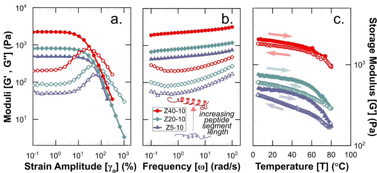
Figure 4. Rheological characterization of 10 wt% hydrogels with varying peptide segment length. a. Strain amplitude and b. frequency responses, wherein filled symbols indicate storage moduli ( G' ) and open symbols indicate loss moduli ( G'' ). c. Storage moduli during temperature ramps performed at \omega = 1 rad/s, with filled and open symbols corresponding to heating and cooling steps, respectively. Full datasets for amplitude and frequency sweeps are given in Figure S6 , and for temperature ramps in Figures S11-13 .
