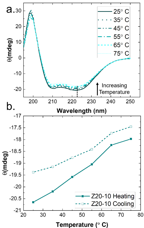
Figure 7: Temperature modulated CD spectra of Z20-10. a. Full wavelength scan shows \alpha -helical secondary structure is maintained over the entire temperature range; only very slight melting can be observed. b. Monitoring the peak intensity at 222 nm reveals hysteresis in secondary structure recovery in a heating/cooling cycle. Points are taken from the temperature scans shown in a.
