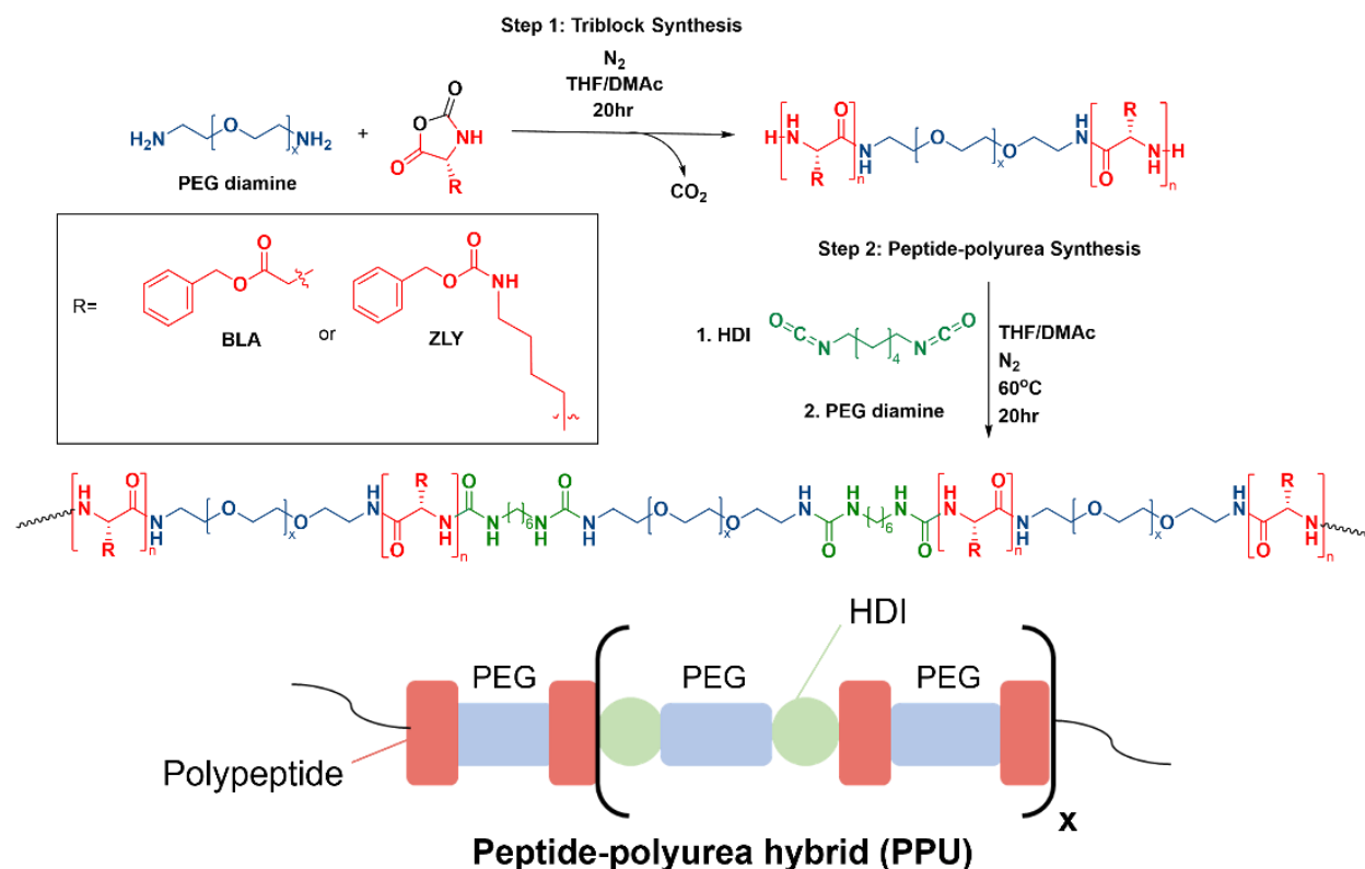
Figure 1: Overall reaction scheme of PPU hybrids and polymer structure
