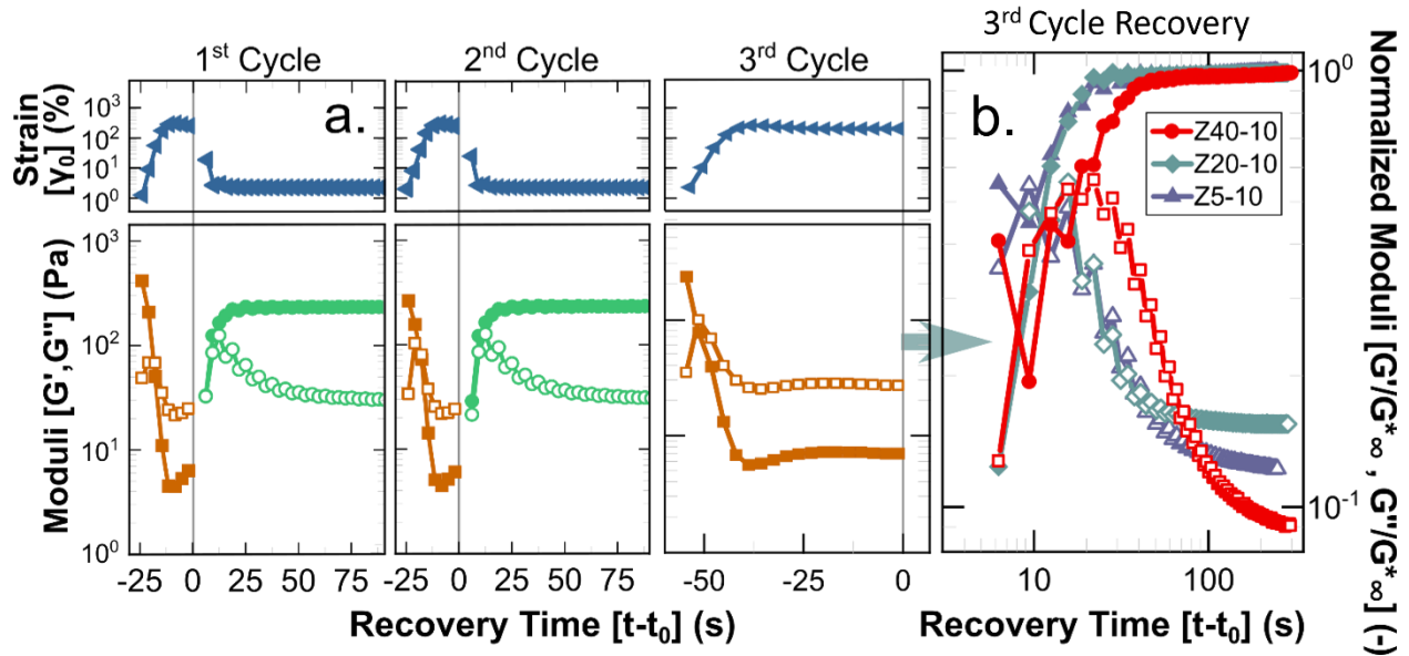
Figure 6: Results of simulated injection experiments. a. three injection-recovery cycles performed for 5 wt% Z20-10 hydrogel. Recovery time is defined as the experimental time ( t ) relative to the cessation of a non-linear oscillatory strain (ending at t_0 ). The recovery period from the 3 rd cycle for all 5 wt% hydrogels is shown in b., wherein filled and open symbols indicate G' and G'' , respectively. Moduli have been normalized by the value of the complex modulus at full recovery ( G^*_{\infty} ).
