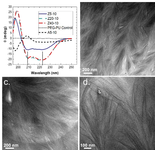
Figure 3. a. CD Spectra of peptide-PEG polyureas. All measurements were taken at 37 °C at a concentration of 2 mg/mL ( i.e. , 0.2 wt%) of polymer in water. Z5-10, Z20-10, and Z40-10 all exhibit strong alpha helical patterns, with a positive cotton band present at 195 nm and characteristic negative peaks appearing at 208 and 222 nm, indicated with dashed lines. Cryo-TEM images of b. Z5-10, c. Z20-10 and d. Z40-10 hydrogels. Dense networks of fibril structures can be observed in all samples. All samples were prepared at a concentration of 10 wt% polymer in water.
