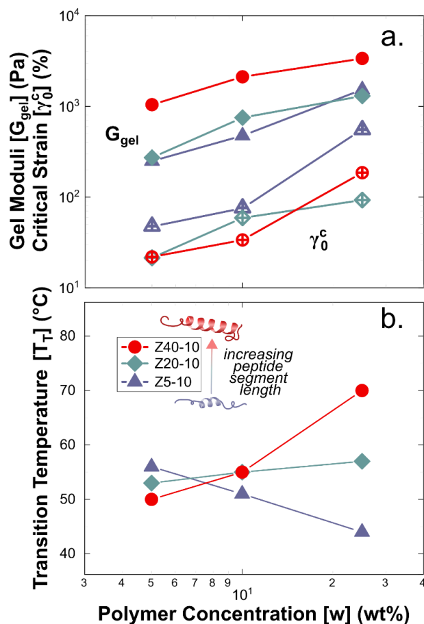
Figure 5. Summary of the rheology of PPU hydrogels as a function of concentration and peptide segment length. a. G_{gel} (filled symbols) and \gamma_0^c (open symbols). b. Transition temperature measured under increasing temperature at a frequency of 100 rad/s.
