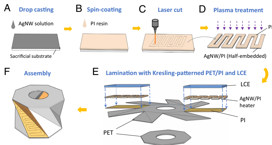
Fig. 2. Fabrication process of the Kresling unit with thermal bimorph actuators. (A) Drop casting of AgNWs on top of a sacrificial substrate. (B) Spin-coating of PI resin on top of the AgNW network. (C) Laser cutting the cured AgNW/PI composite film. (D) Peeling off the serpentine patterned AgNW/PI heater for plasma treatment. (E) Laminating the LCE film and patterned PET/PI sheet with the AgNW/PI heater sandwiched in between. (F) Assembly of the Kresling unit with integrated actuators.
