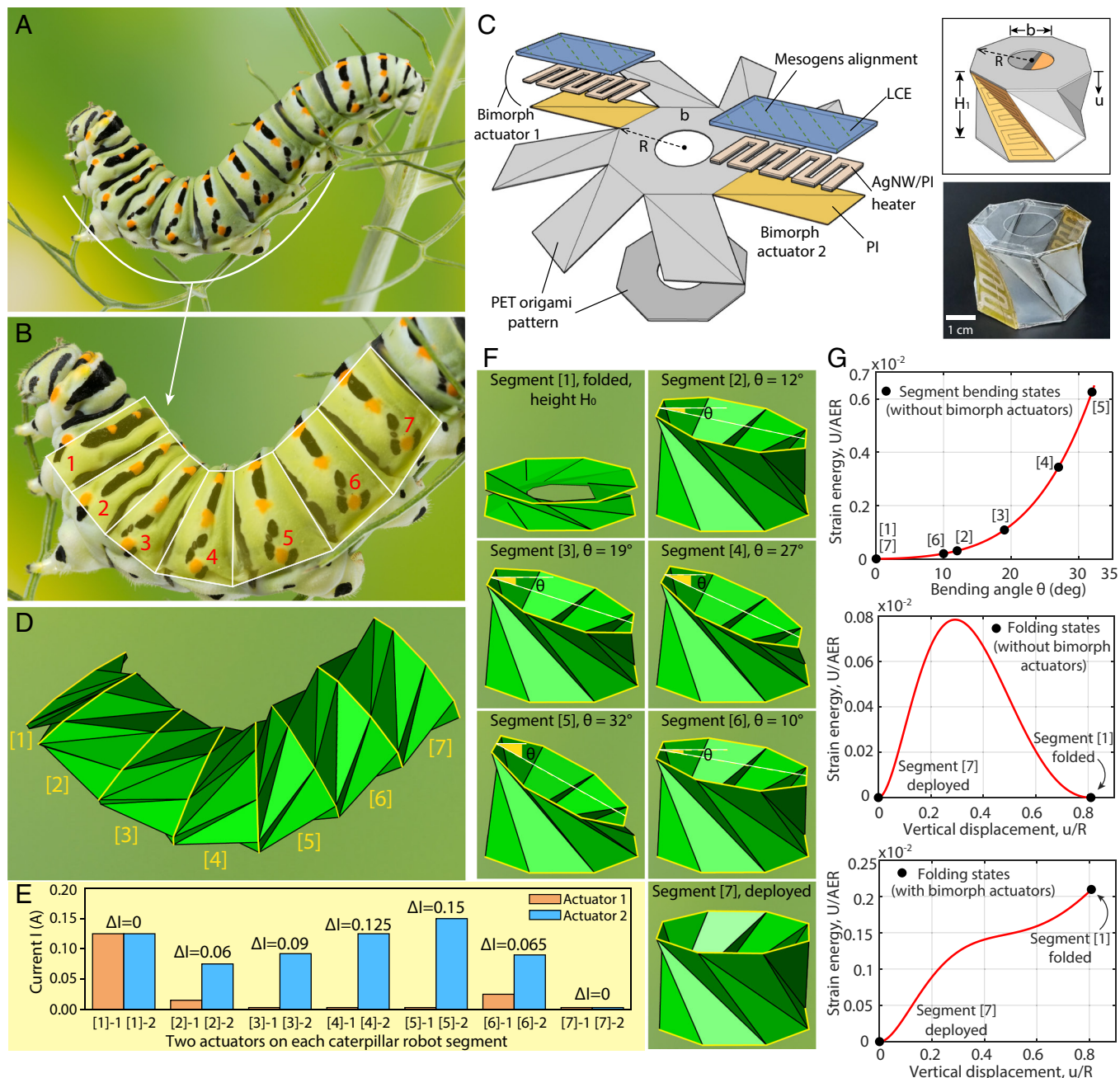
Fig. 1. Lepidoptera larva-inspired Kresling soft robot with thermal bimorph actuators. (A) Photograph of a late fifth instar P. zelandica larva (caterpillar) in a curved configuration with local bending. (B) Body segments of the caterpillar marked from 1 to 7 showing different levels of local contraction and bending. (C) Exploded view of the robot segment composed of electrothermal bimorph actuators integrated with the origami pattern. Insets show the Kresling pattern (Top) and the physical realization (Bottom). Here, LCE denotes liquid crystal elastomer, AgNWs are silver nanowires, PI is polyimide, and PET is polyethylene terephthalate (thermoplastic polymer resin). The symbols H_1 , b , and R denote the height of the deployed Kresling unit, the edge length, and the circumradius of the top octagon plane, respectively. (D) Simulated origami robot including multiple coactive Kresling units mimicking the deformed configuration of the caterpillar. (E) Current applied to the two actuators on each Kresling unit to induce the deformed configuration in (D). (F) Deformed Kresling units with various configurations corresponding to the robot segments. The symbols H_0 and \theta denote the height of the folded Kresling unit and the bending angle between the top and bottom octagon planes, respectively. (G) Top—The stored strain energy of the Kresling origami unit without bimorph actuators of (C) versus bending angle; Middle—strain energy of the origami design without bimorph actuators of (C) versus vertical displacement of any vertices on the top octagon plane; Bottom—strain energy stored in the unit with integrated bimorph actuators of (C) versus vertical displacement. The strain energy ( U/AER ), and displacements ( u/R ) are normalized in the numerical simulation based on the bar-and-hinge method. Here, A and E denote the cross-sectional area and Young's modulus of the bar element, respectively. Those numeric labels (within brackets) refer to the seven configurations of the robot segments in (F).
