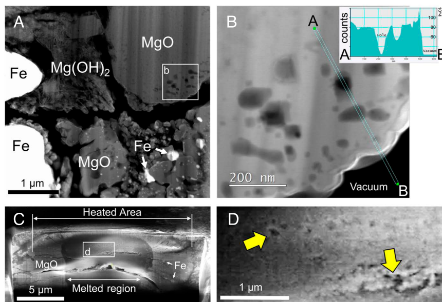
Fig. 4. STEM ( A and B ) and SEM ( C and D ) images of the heated areas in the samples recovered from run #31-003 (11.5 GPa and 3,820 K) and #26-009 (26 GPa and 4,870 K), respectively ( SI Appendix, Table S1 ). ( A ) An FIB section shows some of the phases found in XRD. The small bright grains are bcc Fe metal (labeled as Fe) converted from fcc FeH x during decompression (34). The diffraction pattern for the converted Fe metal can be found in SI Appendix, Fig. S7 . The Fe grains in the left side are not heated. ( B ) Bubble-shaped structures are found along the edge of MgO grains (a white box in A ). An intensity line profile between point A and point B is shown in the inset. ( C ) A cross-section of the laser-heated area in the sample foil was made in FIB to reveal the structures. The center of the heated area contains more MgO and the surrounding area contains more Fe metal. Some Fe metal may migrate during melting along the radial thermal gradients. ( D ) A magnified image (a white box in C ) reveals the bubble-shaped structures (highlighted by yellow arrows) within the heated area, similar to the ones observed in ( B ) but in larger sizes (note the scale difference).
