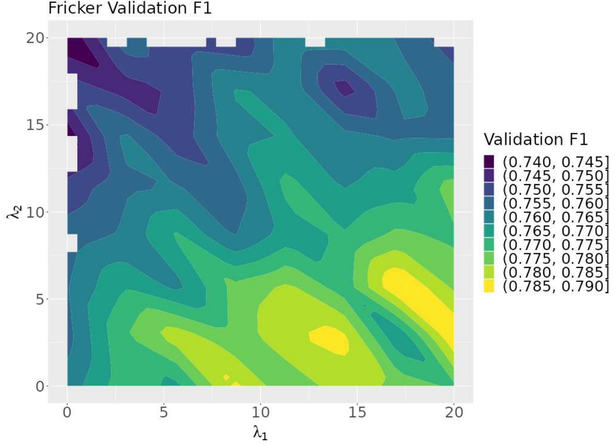
Fig. 12. Validation F1 as a function of \lambda_1 and \lambda_2 .
