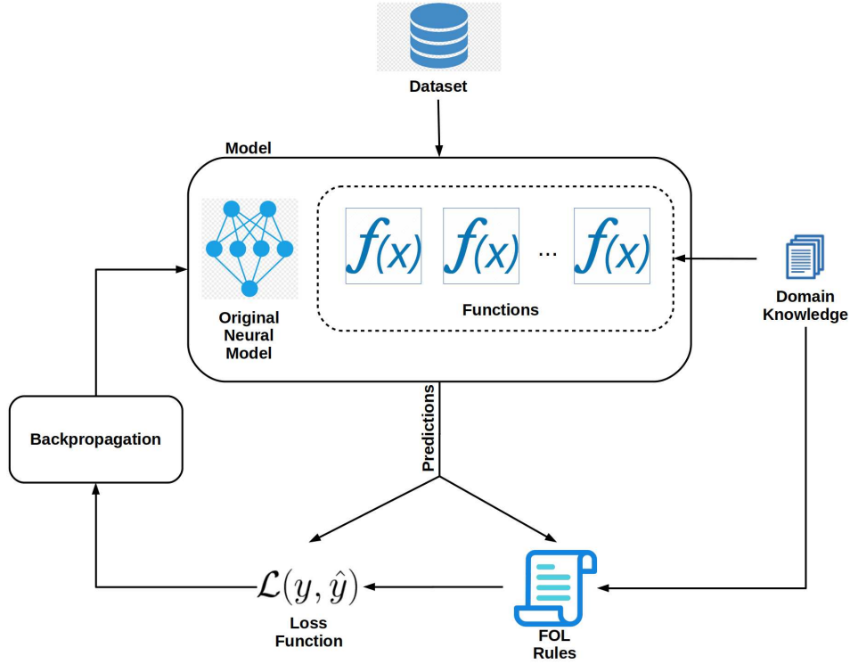
Fig. 2. Model modifications needed to create a neuro-symbolic model.
