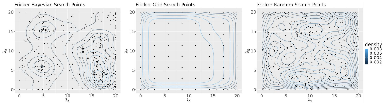
Fig. 10. The density plots of the points selected by each search algorithm.
