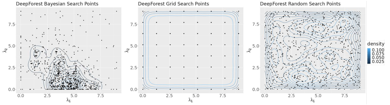
Fig. 5. Contour plots of the points selected by each algorithm for all seeds.
