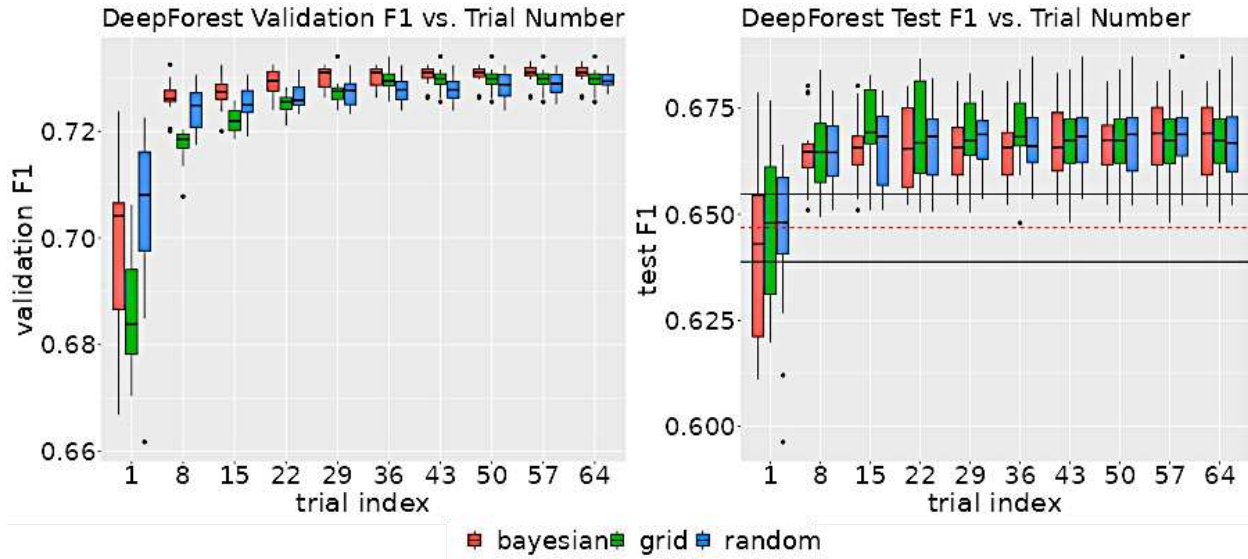
Fig. 6. The left graph shows the distribution of validation scores as a function of the number of trials for each search method. The right graph shows the distribution of test F1 scores as a function of the number of trials for each method. The test F1 score was determined by evaluating the model on the test set using the hyperparameters associated with the highest validation score at the listed trial index. The black horizontal lines on the test F1 graph show the upper and lower 95% confidence intervals for non-neuro-symbolic DeepForest. The dashed red line is the mean test set F1 score of the non-neuro-symbolic model.
