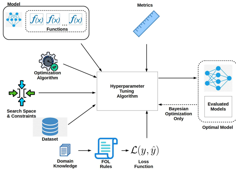
Fig. 1. Framework system overview.
