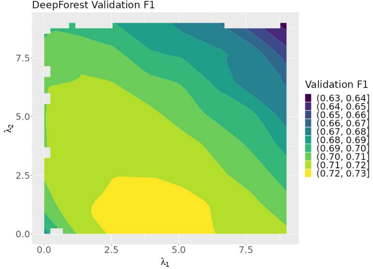
Fig. 7. A contour plot of the validation F1 scores over the search space.
