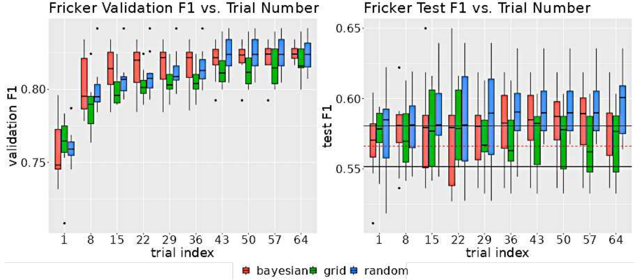
Fig. 11. The left graph shows the distribution of the validation F1 scores for the indicated number of trials for each search algorithm. The right graph shows the distribution of test F1 scores for the indicated number of trials. The hyperparameters selected for the test model were the ones corresponding to the highest validation F1 score up to the indicated trial. In the test graph, the two horizontal black lines indicate the 95% confidence intervals for non-neuro-symbolic test set F1 scores. The horizontal dashed red line indicates the mean of non-neuro-symbolic model test set F1 scores.
