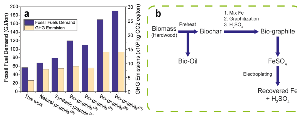
Figure 4. LCA results. a) Life-cycle fossil fuel consumption (GJ) and greenhouse gas emissions ( \times 10^3 kg CO 2 e) per metric ton graphite for different synthesis methods. b) System boundary for our bio-graphite synthesis method.
