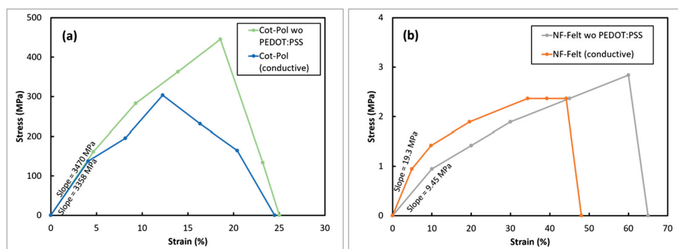
Figure 3. Stress vs. strain responses from (a) Cot-Pol and (b) NF-Felt string electrodes.
