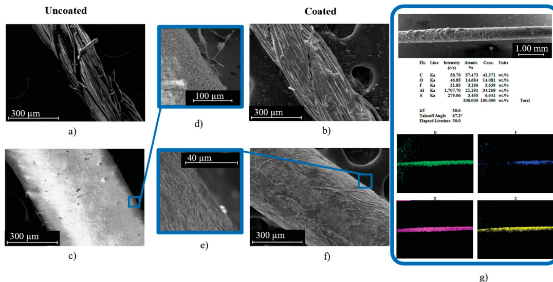
Figure 2. (a) Cot-Pol string for fiber observation (uncoated) at 300 μm; (b) Cot-Pol string for string observation (coated); (c) NF-Felt string for fiber observation (uncoated) at 300 μm; (d) surface close up of uncoated NF-Felt; (f) NF-Felt string for string observation (coated); (e) surface close up of coated NF-Felt; (g) EDS analysis of coated NF-Felt electrode.
