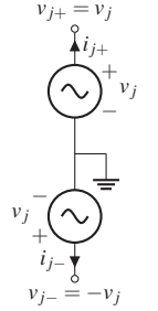
Fig. 3: Differential spin node.
