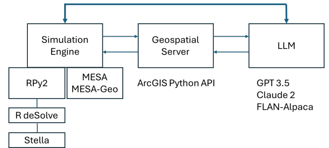
Figure 2: The overall architecture of LLM integration with simulation systems
