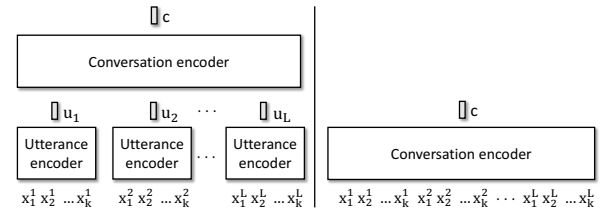
Figure 1: Left: Coarse-grained integration of dialog history. Here, x_i^j represents the i^{th} token in the j^{th} utterance in the dialog. Each utterance is encoded separately into a representation u_j and the sequence \{u_j\}_{j=1}^L is passed to another sequence encoder to get the context representation c . Right: Fine-grained integration of dialog history. The entire sequence of tokens in the conversation \{\{x_i^j\}_{i=1}^k\}_{j=1}^L is passed as a single contiguous sequence to the conversation encoder.
