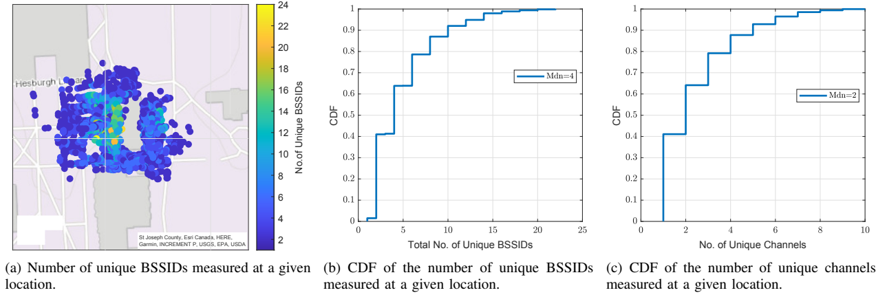
Fig. 8: CDF plots for walking measurements: Number of unique BSSIDs and channels.
