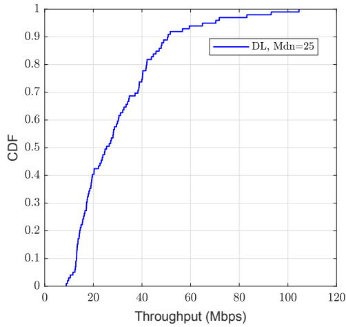
Fig. 5: CDF of downlink throughput at 6 GHz.
