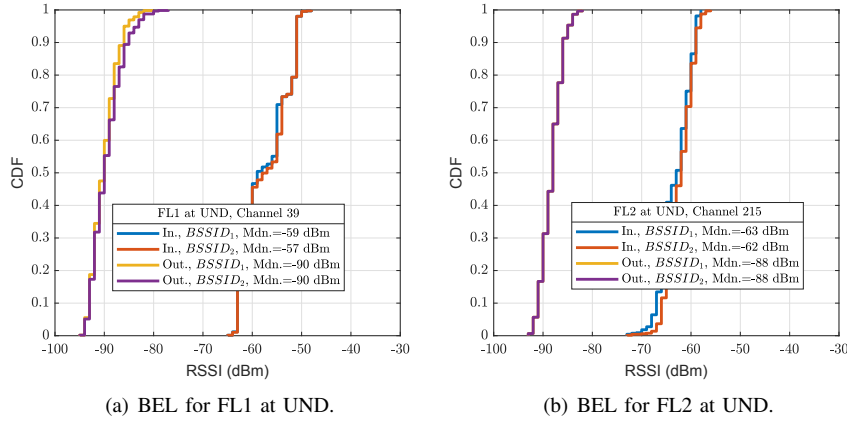
Fig. 9: BEL near a solid brick wall at two different measurement environments.
