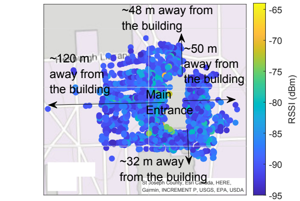
Fig. 3: Outdoor RSSI at 6 GHz via walking measurements.
