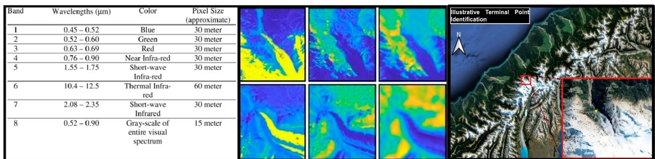
Figure 5. (Left) Multispectral band information for images taken by Landsat 7. (Middle) Top Franz Josef; Bottom: Gorner; from left to right: Band 1, Band 5, Band 6 shown in false colors. (Right) Terminal Identification process.
