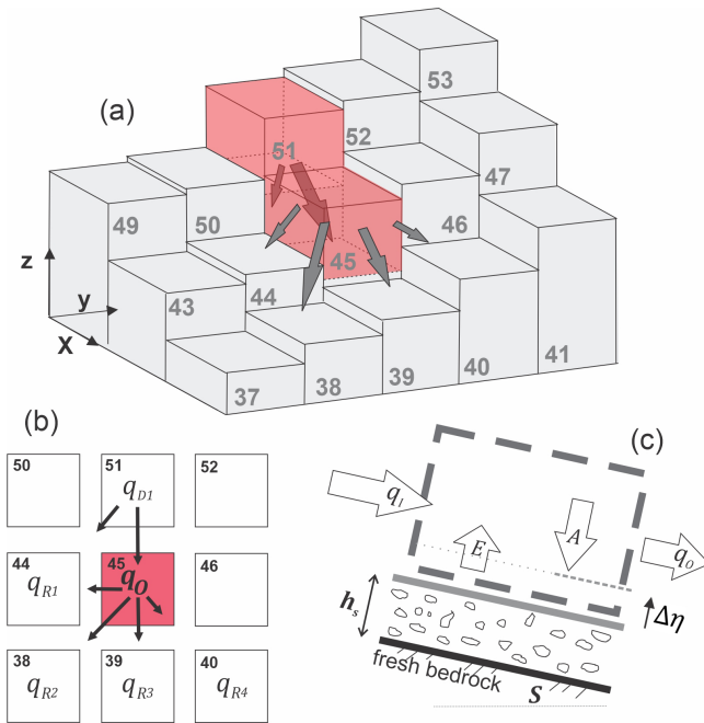
Figure 3. (a) Three-dimensional illustration of iteration t = 0 in Fig. 2, showing initial source material nodes (represented by red cells) and flux towards downslope nodes. (b) Distribution of q_0 to downslope nodes 38, 39, 40, and 44; (c) illustration of mass continuity applied to any node that receives a debriton.
