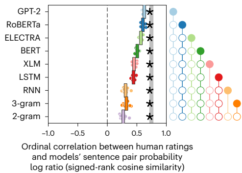
Fig. 4 | Ordinal correlation of the models' sentence probability log ratios and human Likert ratings. For each sentence pair, model prediction was quantified by \log \frac{p(s^1|m)}{p(s^2|m)} . This log ratio was correlated with the Likert ratings of each particular participant, using signed-rank cosine similarity (Methods). This analysis, taking all trials and human confidence level into account, indicates that GPT-2 performed best in predicting human sentence probability judgements. However, its predictions are still significantly misaligned with the human choices. See the caption to Fig. 1 for details on the visualization convention.
