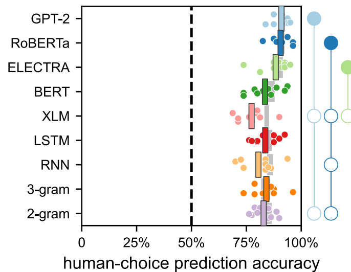
Extended Data Fig. 6 | Model prediction accuracy for pairs of natural and synthetic sentences, evaluating each model across all of the sentence pairs in which it was targeted to rate the synthetic sentence to be less probable than the natural sentence. The data binning applied here is complementary to the one used in Fig. 3b, where each model was evaluated across all of the sentence pairs in which it was targeted to rate the synthetic sentence to be at
