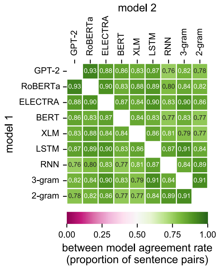
Extended Data Fig. 2 | Between-model agreement rate on the probability ranking of the 90 randomly sampled and paired natural sentence pairs evaluated in the experiment. Each cell represents the proportion of sentence
