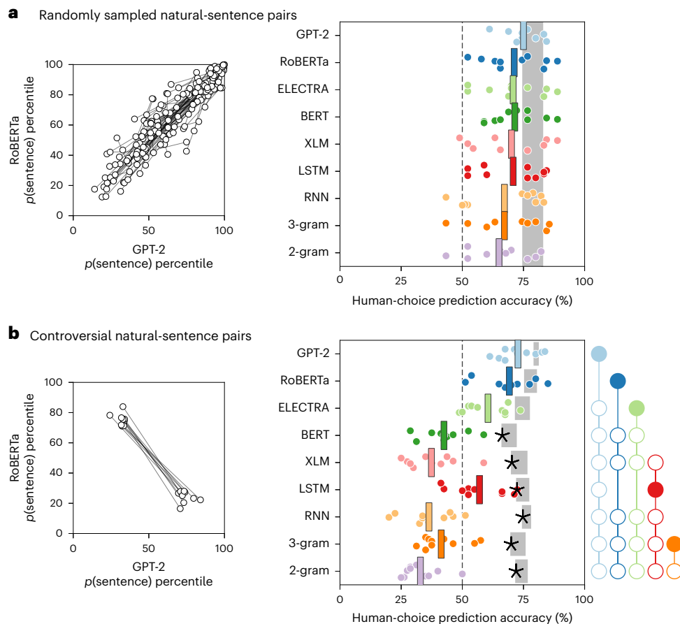
Fig. 1 | Model comparison using natural sentences. a, Left: percentile-transformed sentence probabilities for GPT-2 and RoBERTa (defined relative to all sentences used in the experiment) for randomly sampled pairs of natural sentences. Each pair of connected circles depicts one sentence pair. The two models are highly congruent in their rankings of sentences within a pair (lines have an upward slope). Right: accuracy of model predictions of human choices, measured as the proportion of trials in which the same sentence was preferred by both the model and the human participant. Each circle depicts the prediction accuracy of one candidate model averaged across a group of ten participants presented with a unique set of trials. The coloured bars depict grand averages across all 100 participants. The grey bar is the noise ceiling, with its left and right edges being lower and upper bounds on the grand-average performance an ideal model would achieve (based on the consistency across human subjects). There
