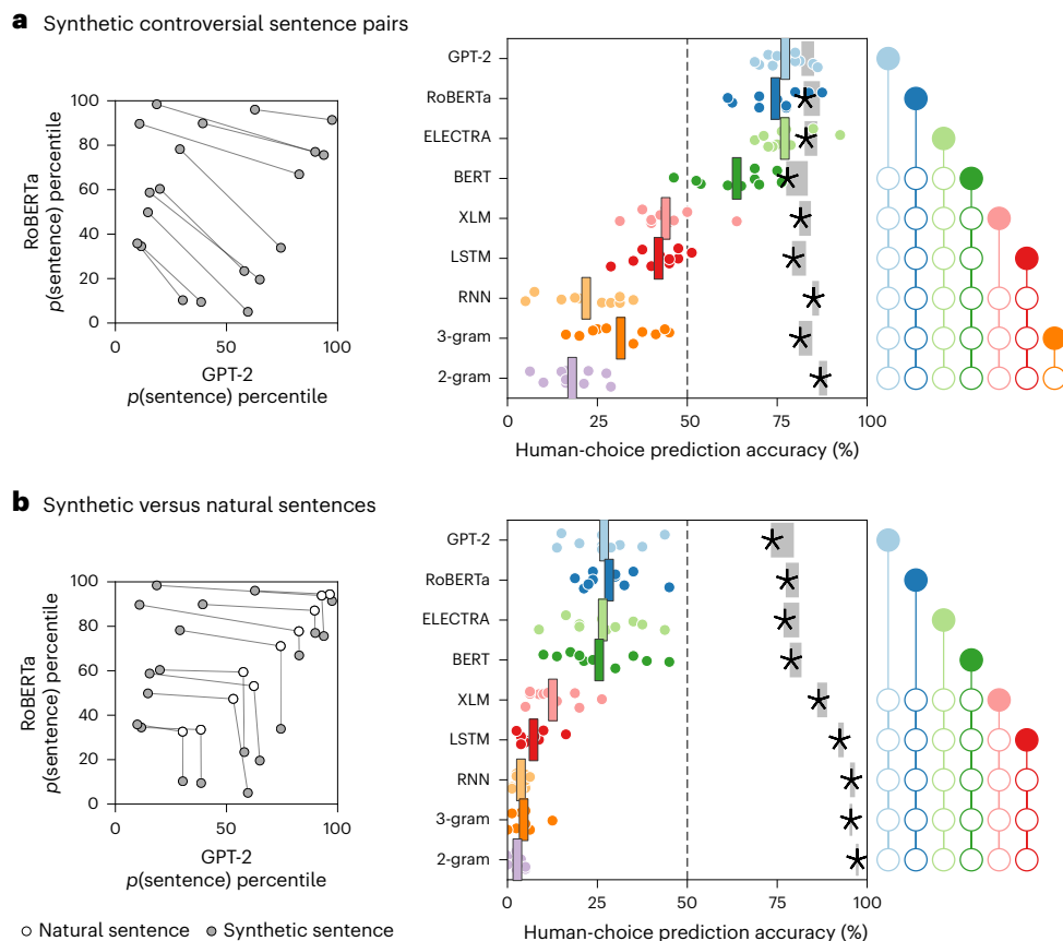
Fig. 3 | Model comparison using synthetic sentences. a, Left: percentile-transformed sentence probabilities for GPT-2 and RoBERTa for controversial synthetic sentence pairs. Each pair of connected circles depicts one sentence pair. Right: model prediction accuracy, measured as the proportion of trials in which the same sentence was preferred by both the model and the human participant. GPT-2, RoBERTa and ELECTRA significantly outperformed the other models (two-sided Wilcoxon signed-rank test, controlling the false discovery rate for all 36 model comparisons at q < 0.05 ). All of the models except for GPT-2 were found to perform below the noise ceiling (grey) of predicting each participant's choices from the majority votes of the other participants (asterisks indicate significance—two-sided Wilcoxon signed-rank test, controlling the false discovery rate for nine comparisons at q < 0.05 ). b, Left: each connected
