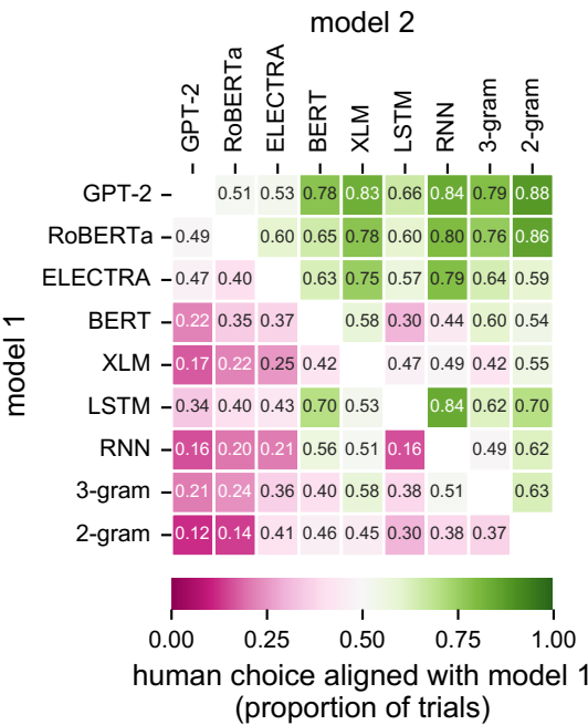
Extended Data Fig. 3 | Pairwise model comparison of model-human consistency. For each pair of models (represented as one cell in the matrices above), the only trials considered were those in which the stimuli were either selected (a) or synthesized (b) to contrast the predictions of the two models. For these trials, the two models always made controversial predictions (that is, one sentence is preferred by the first model and the other sentence is preferred by the
