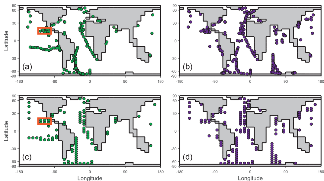
Figure 2. Ocean surface (uppermost ~ 81 m corresponding to the depth of the surface layer in the cGENIE model) sampling locations of \text{IO}_3^- (a) and \text{I}^- (b) field observations after data filtration for freshwater and sediment fluxes. The filtered observations were then gridded according to the cGENIE 36 \times 36 \times 16 framework for model–data comparison of \text{IO}_3^- (c) and \text{I}^- (d). The orange boxes in panels (a) and (c) highlight the grids of the oxygen-deficient zone transect shown in Fig. 7.
