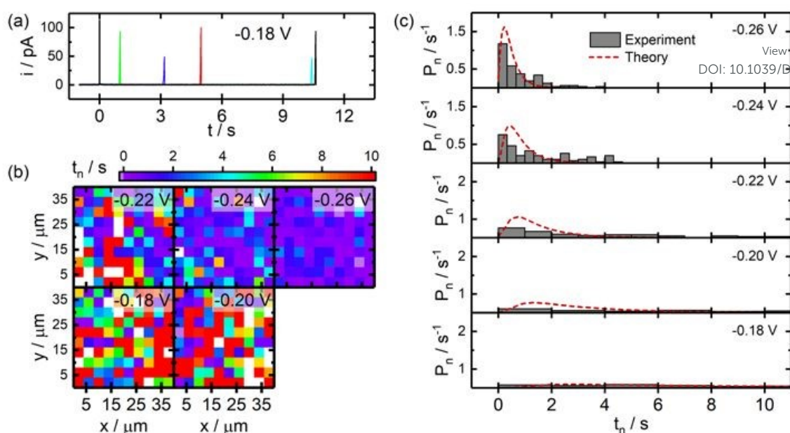
Figure 4: SECCM studies of Ag NP nucleation on ITO electrodes. (a) Example current transients recorded during SECCM experiments at an applied potential of -0.18 V vs. QRCE. (b) Images of measured nucleation times at a series of different applied potentials. (c) Experimental distribution of nucleation times and fits to the time dependent nucleation model. All experiments were carried out using a probe with terminal dimensions of ca. 1 \mu\text{m} filled with an aqueous solution of 0.5 mM \text{AgNO}_3 and 50 mM \text{NaClO}_4 . The theoretical curves in (c) were generated for \chi = 14.4 and k = 2.8 \text{ s}^{-1} .
