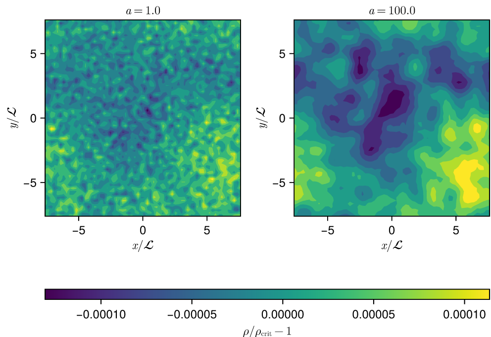
Figure 1: Growth of density perturbations in a scalar field in an expanding background, as the universe's scale factor grows from a = 1.0 to a = 100.0 . The density is measured in units of the universe's critical density \rho_{\text{crit}} . This scenario is similar to that in (Musoke et al., 2020), in which the scalar field is an inflaton fragmenting after the end of primordial inflation.
