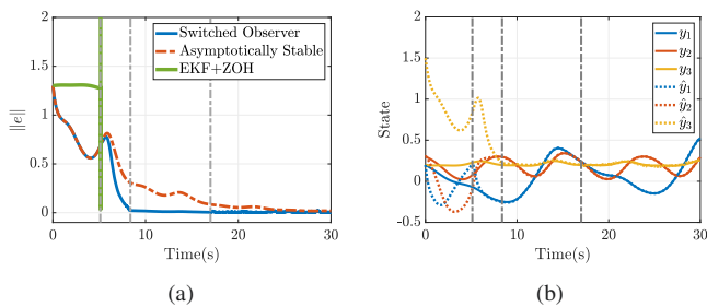
Figure 1. Simulation Results showing (a) Comparison of observers based on error norm. (b) State estimation using switched observer.
