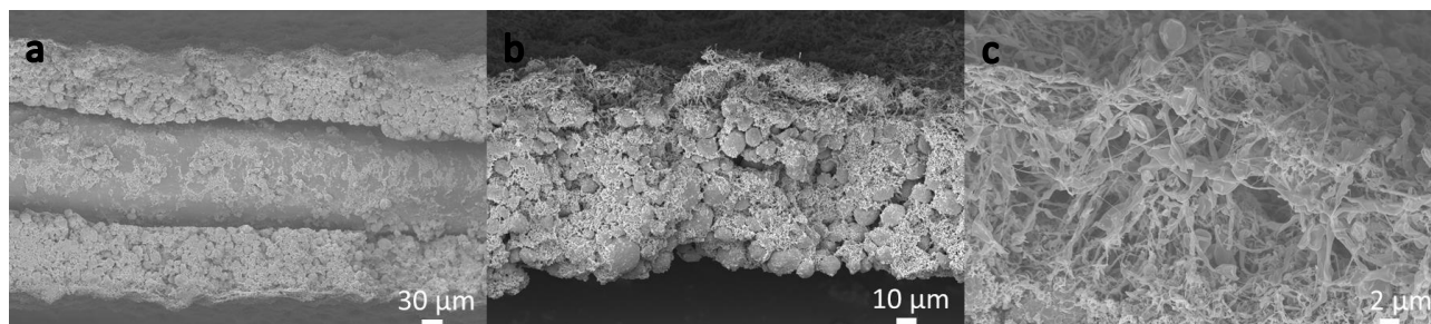
Figure 2(a-c). Cross-sectional SEM images showing (a) top and bottom of fractured PI coated NMC electrode. The middle layer is Al current collector, onto which the cathodic material was deposited. (b) PI coated NMC electrode at 500x with PI layer present on the top surface. (c) PI coating morphology displaying a network of particles with characteristic bead-on-string architectures at 2.5kx magnification.
