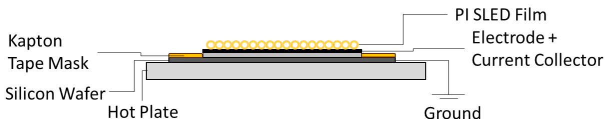
Figure 1. Illustration of the SLED film deposited onto an electrode. The use of a Kapton tape film mask improves coating uniformity and coverage by redirecting the electrostatic field lines of the spray onto the electrode.
