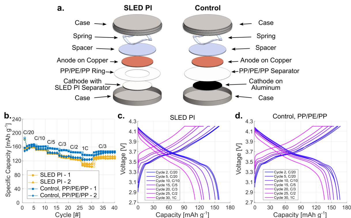
Figure 5. Cycling performance of SLED PI and control full-cells. . (a) Schematic of full-cell assemblies for SLED PI and control cells. (b) Specific capacity as a function of cycle number and C-rate. Hollow markers indicate charge capacity and filled markers indicate discharge capacity. Voltage profiles for the different C-rates for (c) a SLED PI full-cell and (d) a control sample with only a PP/PE/PP separator.
