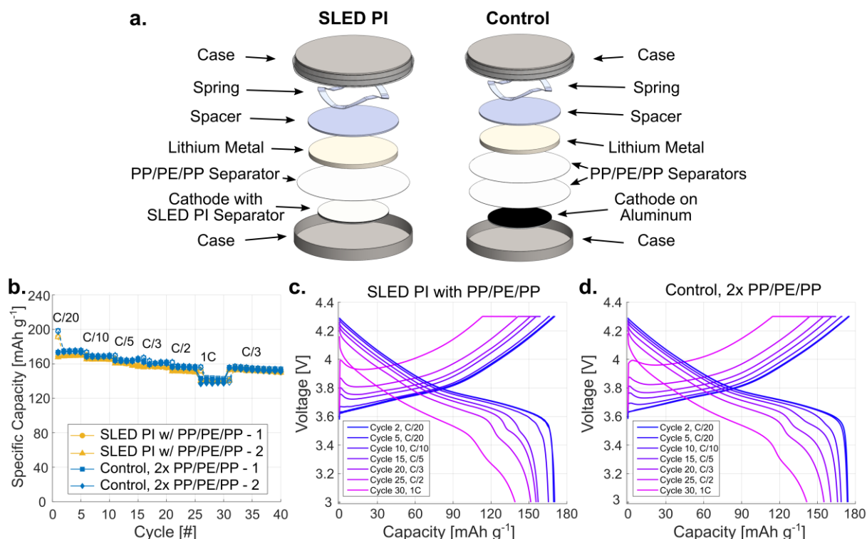
Figure 4. Cycling performance of SLED PI and control half-cells. (a) Schematic of half-cell assemblies for SLED PI and control cells. (b) Specific capacity as a function of cycle number and C-rate. Hollow markers indicate charge capacity and filled markers indicate discharge capacity. Voltage profiles for the different C-rates for (c) a SLED PI half-cell and (d) a control sample with only PP/PE/PP separators.
