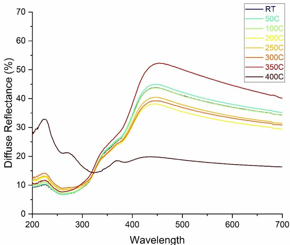
Figure 3. Diffuse reflectance UV-Vis spectra of SLED PI films on a Si substrate, illustrating the impact of temperature on film porosity. The PI was initially sprayed at RT, then thermally treated for ~10 minutes at each temperature increment, followed by RT UV-Vis spectral analysis for each temperature.
